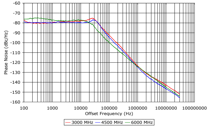
Phase Noise
