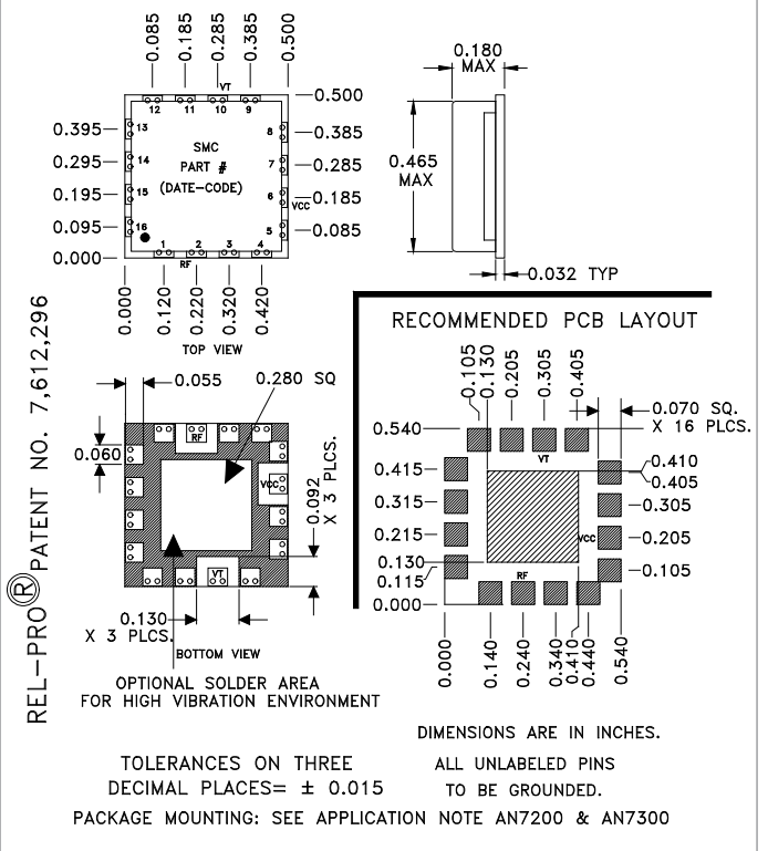
Package # 278LF
