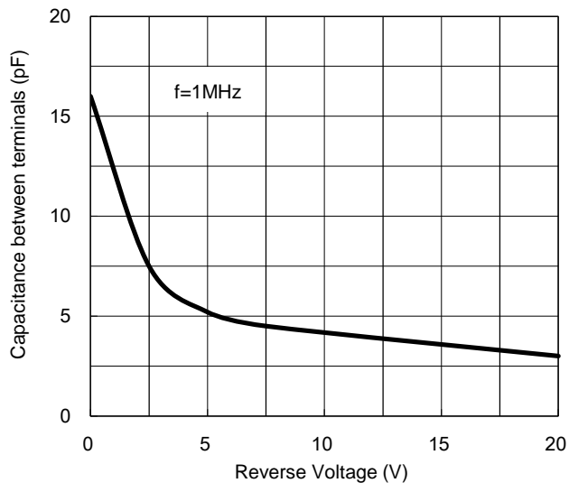
Fig. 3 Capacitance Characteristics
