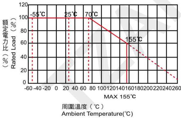
線繞型水泥電阻 Wirewound Cement Type
