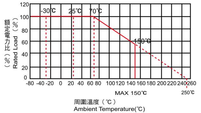
金屬氧化皮膜水泥電阻 Metal Oxide Film Cement Type
