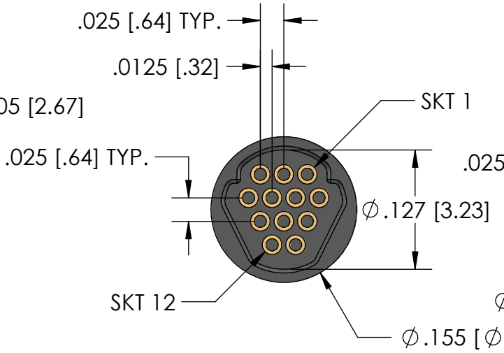
12 POSITION RECEPTACLE
