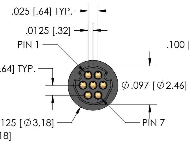
7 POSITION PLUG
