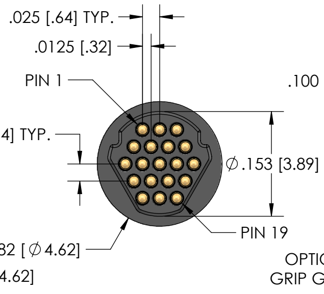
19 POSITION PLUG
