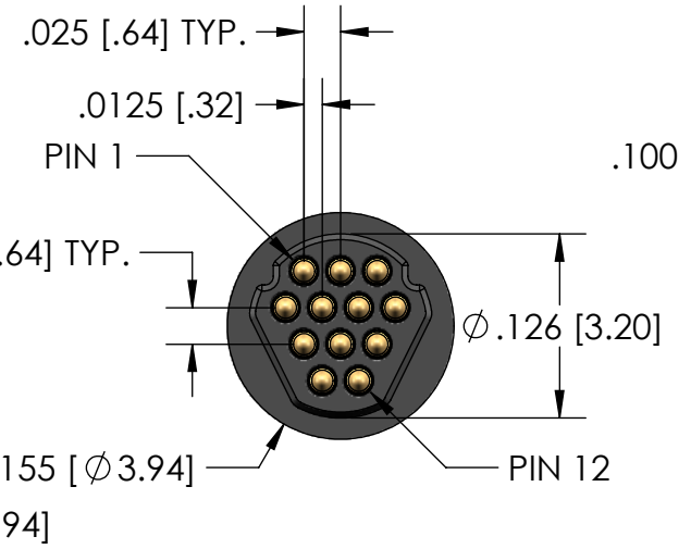
12 POSITION PLUG
