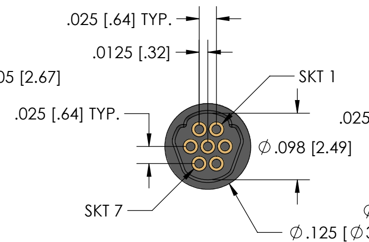
7 POSITION RECEPTACLE
