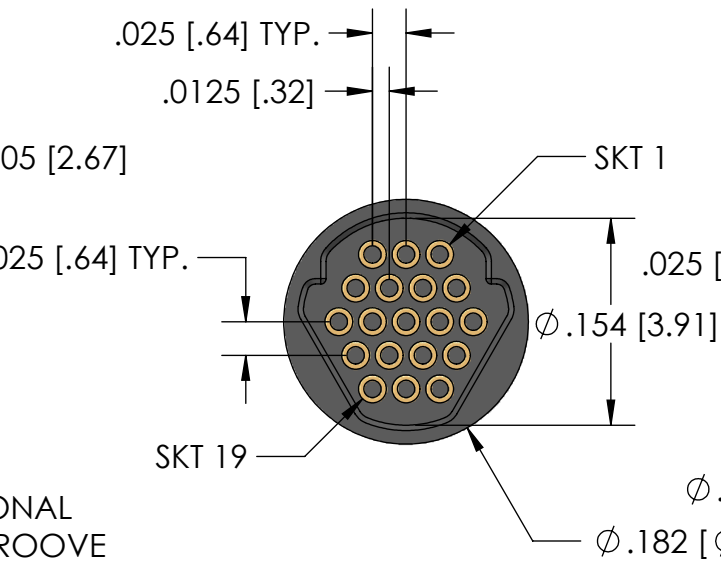
19 POSITION RECEPTACLE
