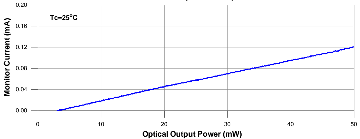
Monitor Current v.s. Optical Output Power
