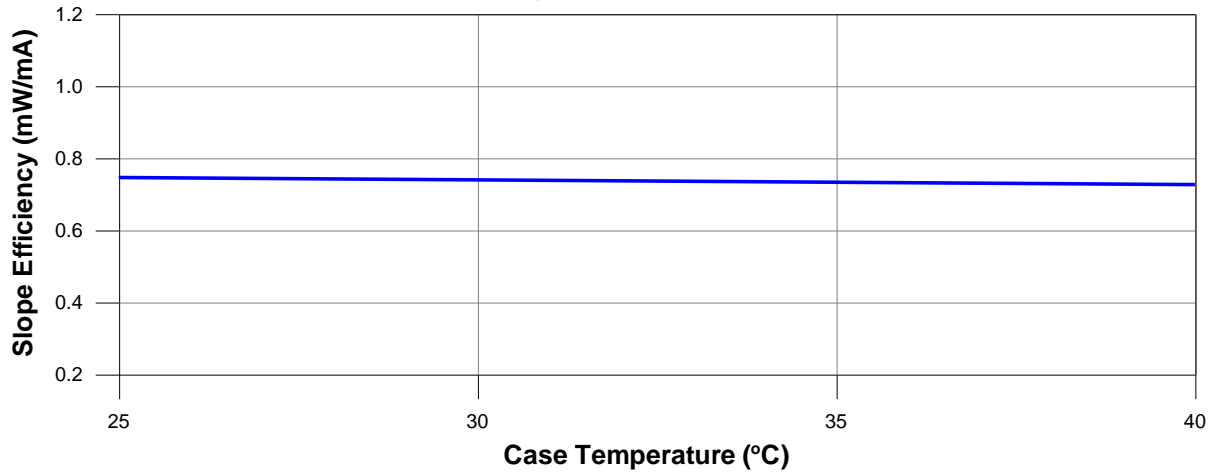
Slope Efficiency v.s. Case Temperature
