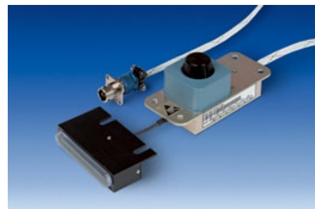
LED Map Lights D947-06-001-004 (Captain) D947-16-001-004 (First Officer)
