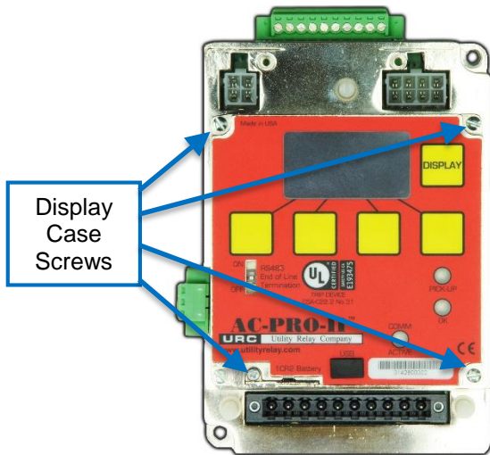
Figure B: Display Case Screw locations
