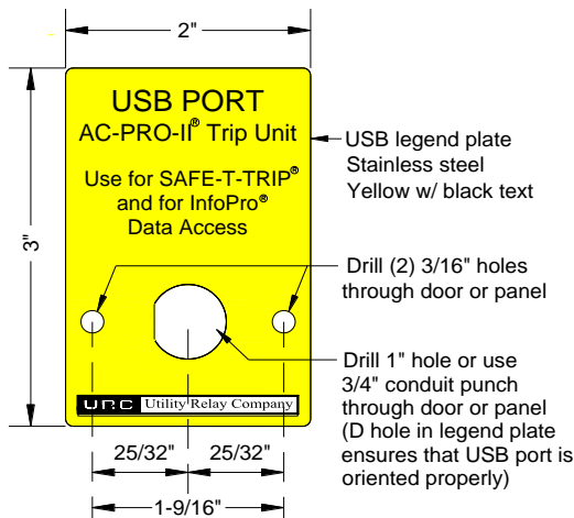
Figure L: USB Extension Plate Drilling
