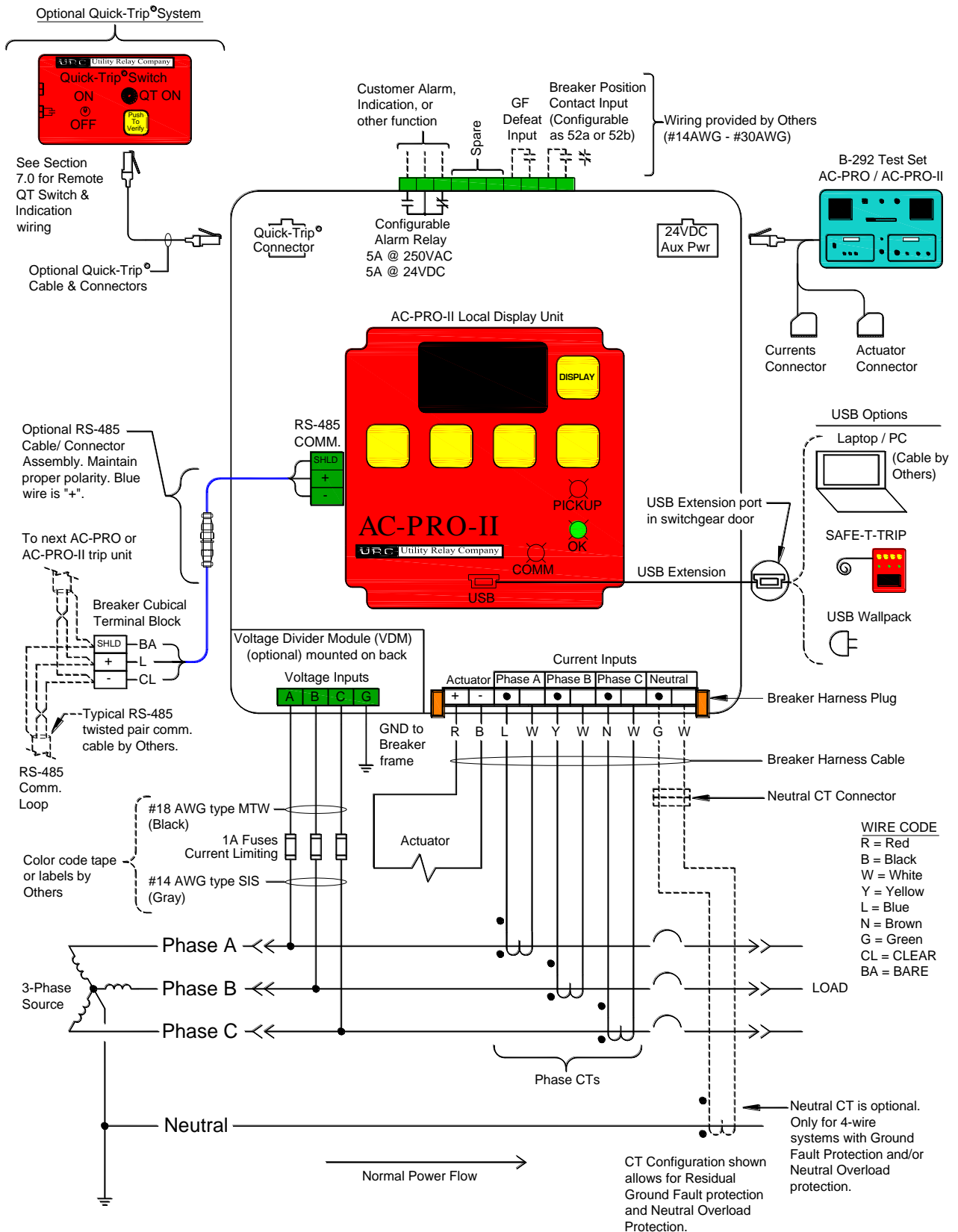
Figure E: AC-PRO-II Typical Wiring Diagram
