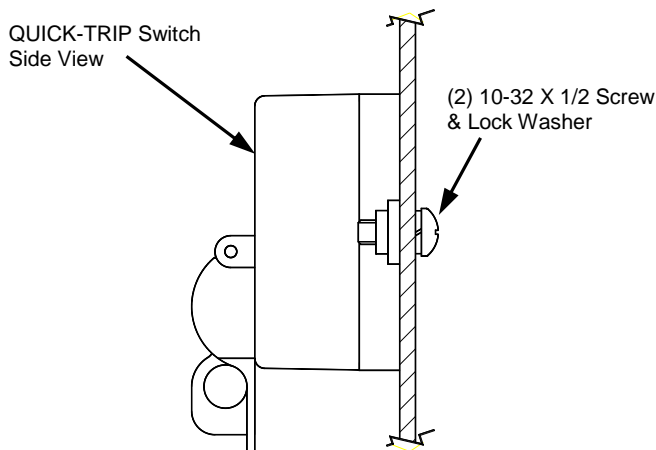
Figure I: QUICK-TRIP Switch Mounting
