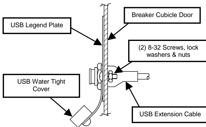
Figure M: USB Extension Plate & Cable Installation
