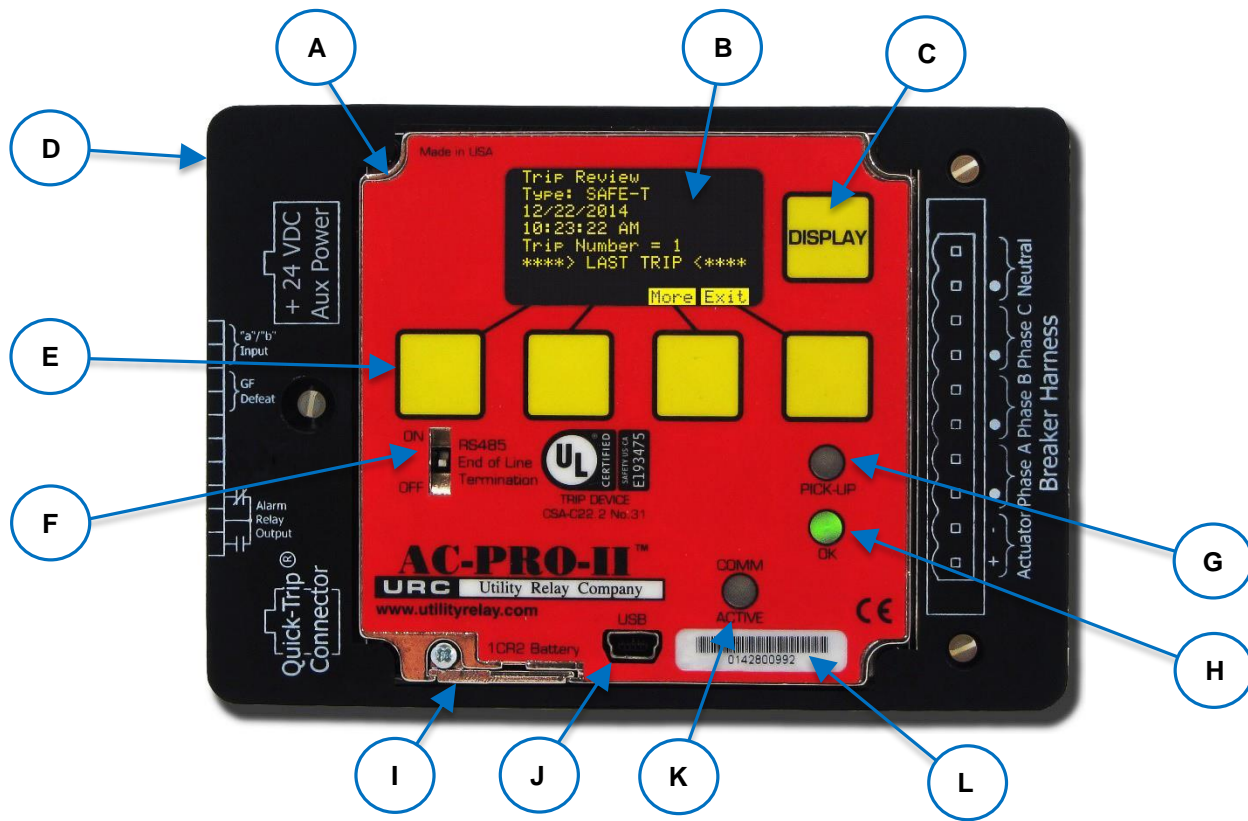
Figure A: AC-PRO-II Front View - Horizontal Configuration (See page 2 for Item descriptions)
