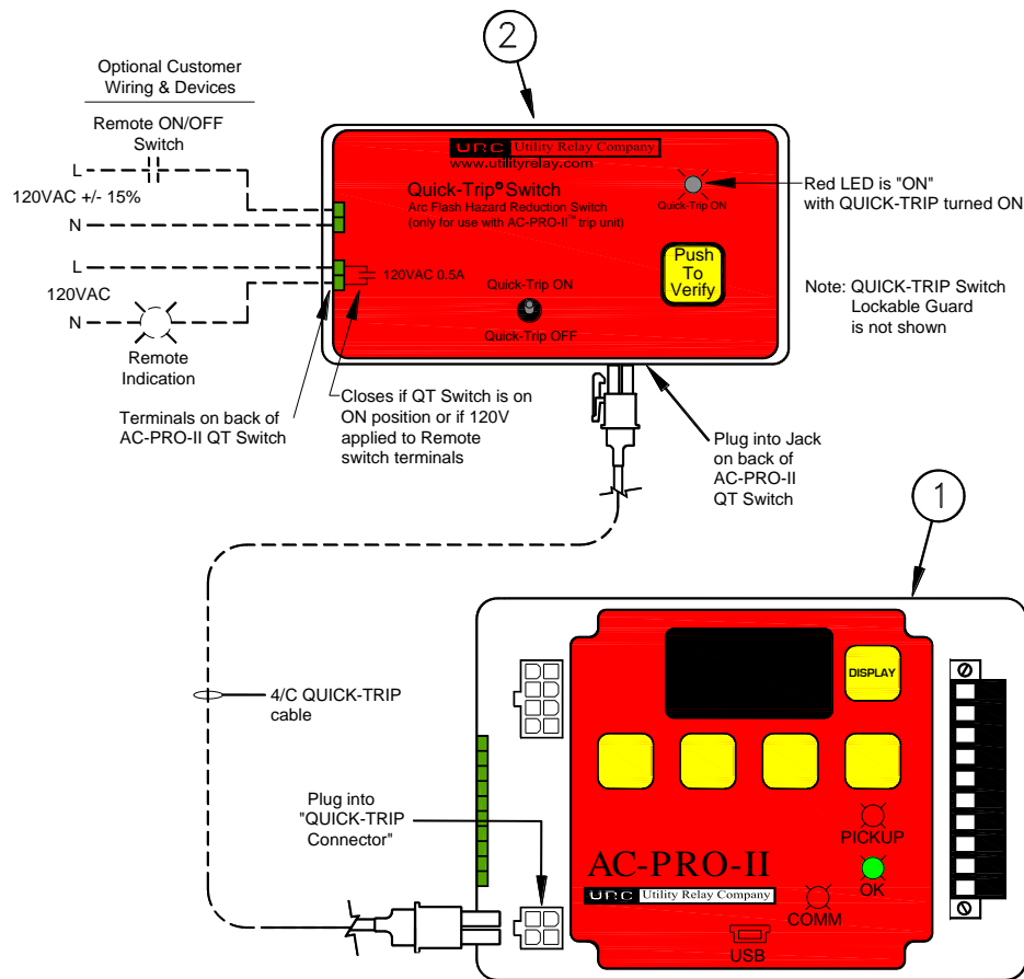
Figure G: QUICK-TRIP System and Connections
