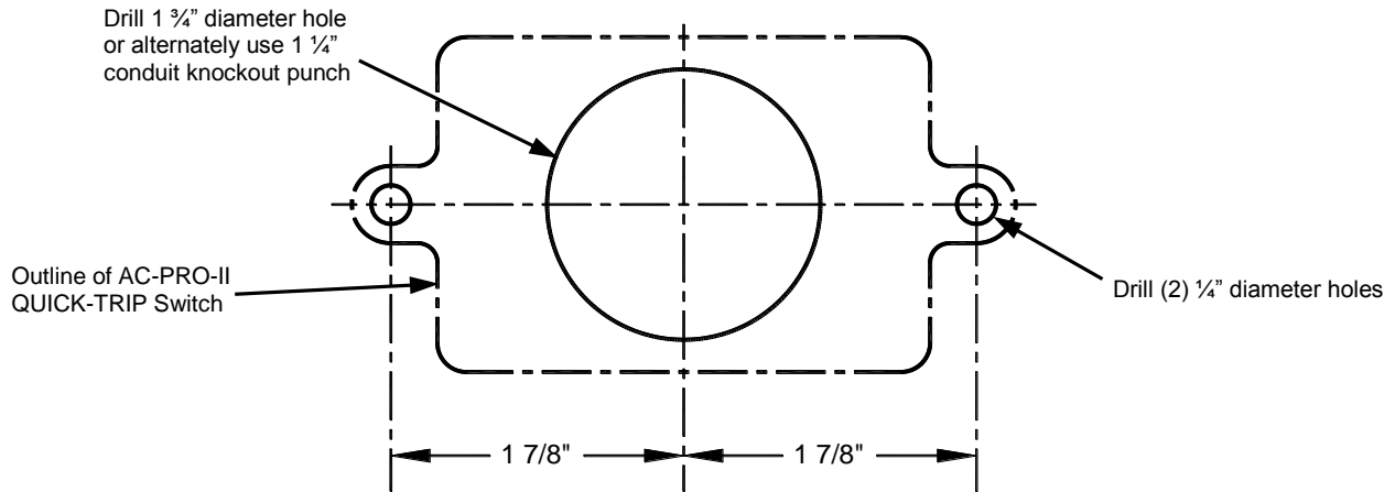
Figure H: AC-PRO-II QUICK-TRIP Switch Drilling Plan
