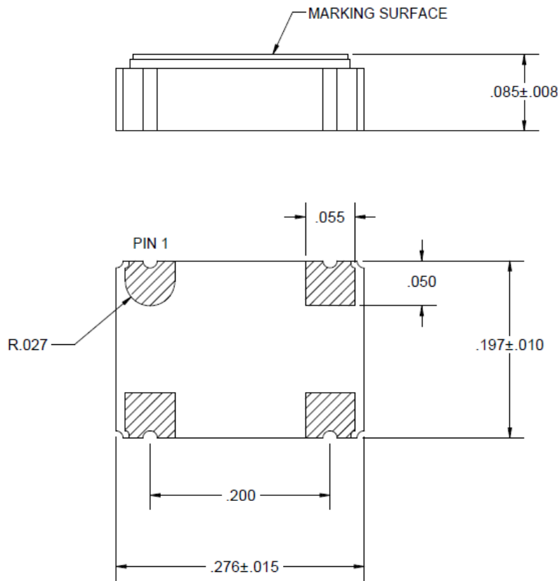
FIGURE 8 Model 1157 Package Outline
