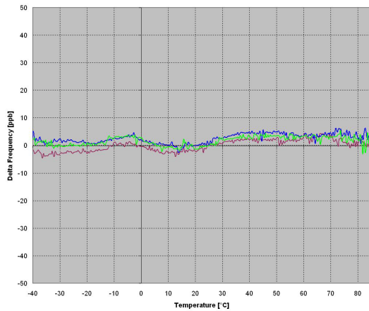
Frequency vs. Temperature TX-503 @ 20MHz
