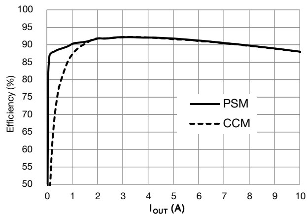
Fig. 4 - Efficiency - PSM vs. CCM (V DD = 3.3 V, V OUT = 1.5 V, V IN = 12 V)
