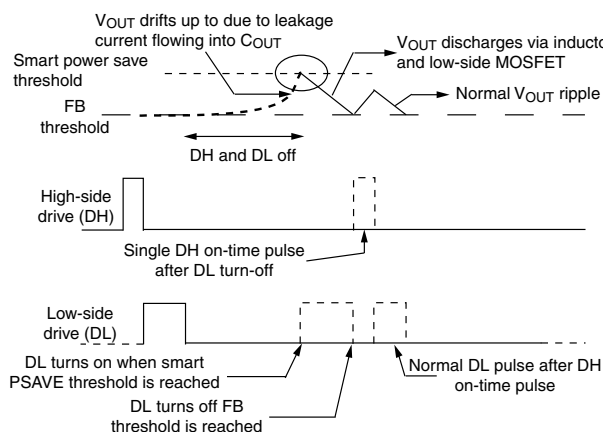
Fig. 29 - Smart Power-Save
