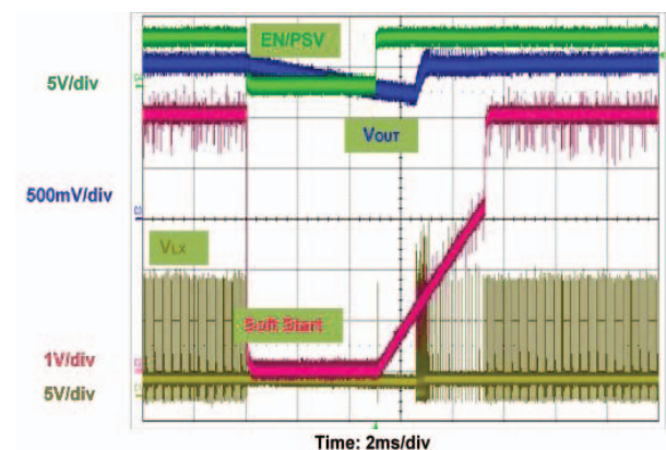
Fig. 14 - Start-Up (Pre-Bias) - EN/PSV ( V_{DD} = 5\text{ V} , V_{IN} = 12\text{ V} , V_{OUT} = 1.5\text{ V} , I_{OUT} = 0\text{ A} )
