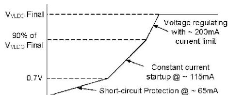
Fig. 33 - LDO Start-Up
