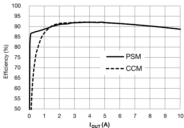
Fig. 5 - Efficiency - PSM vs. CCM (V DD = 5 V, V OUT = 1.5 V, V IN = 12 V)
