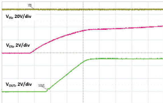
Fig. 23 - Start-Up with EN, Time = 1 ms/div
