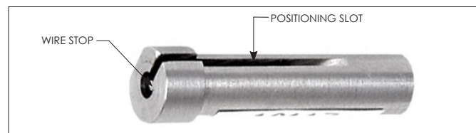
Figure B. Locator positioning slot and wire stop only found on Part # 910 104 127.
