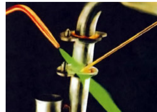
Yellow Stop-Off for Torch Brazing image source: AWS Brazing Handbook P. 238
