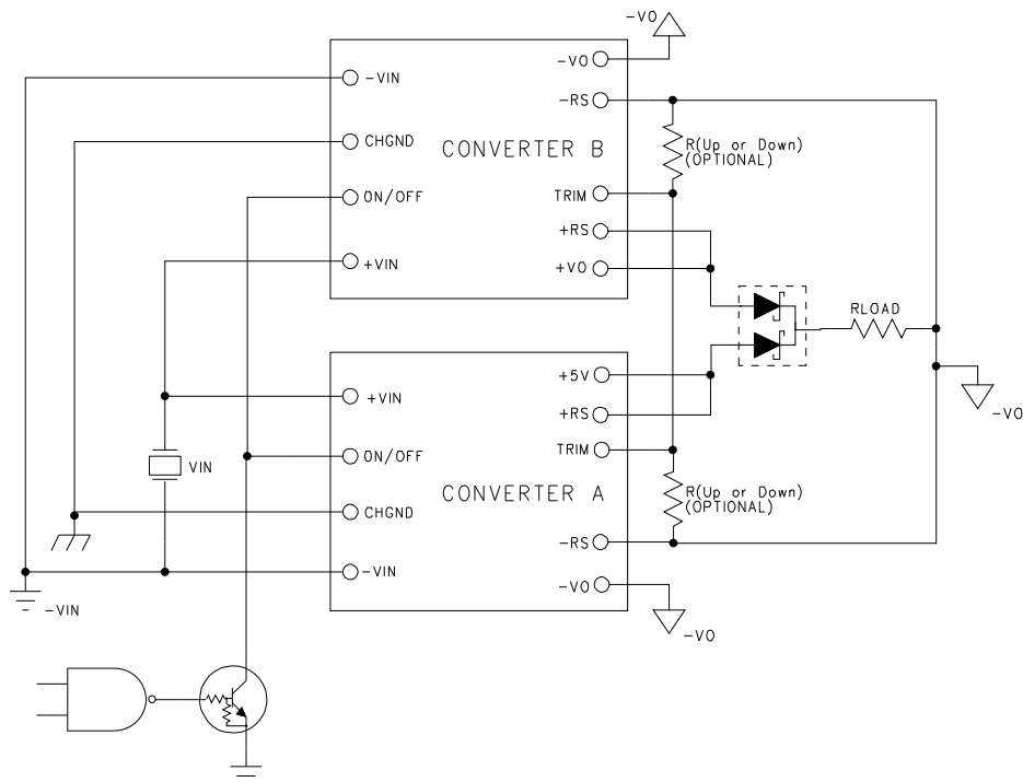
Figure 6: Paralleling Converters
