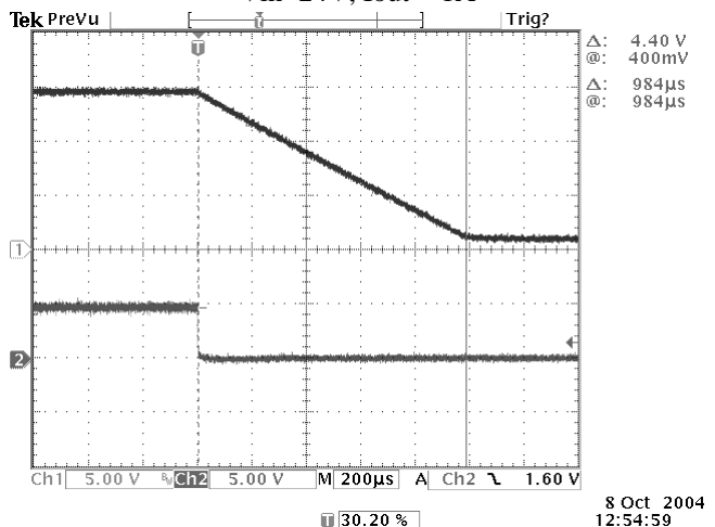
Photo 5: Remote Turn Off Vin=24V, Iout = 1A
