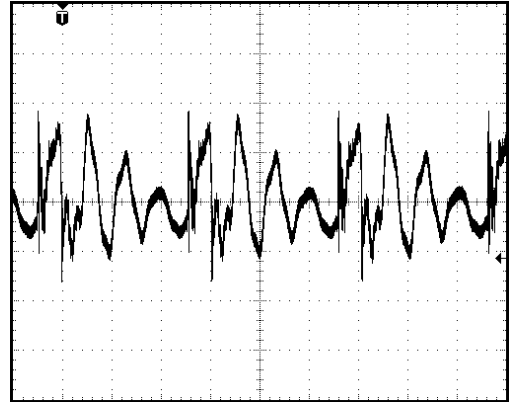
TYPICAL OUTPUT RIPPLE 20mV/div, 1uS/div, full load 75Vin 0.1uF decoupling cap at room temp
