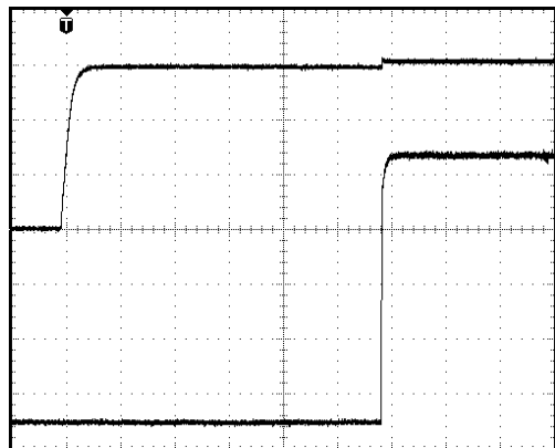
TYPICAL RISE TIME & TURN-ON DELAY USING LOGIC ENABLE 1V/div, 10mS/div (Vout), 2V/div 10mS/div (logic enable) 18Vin, full load at room temp
