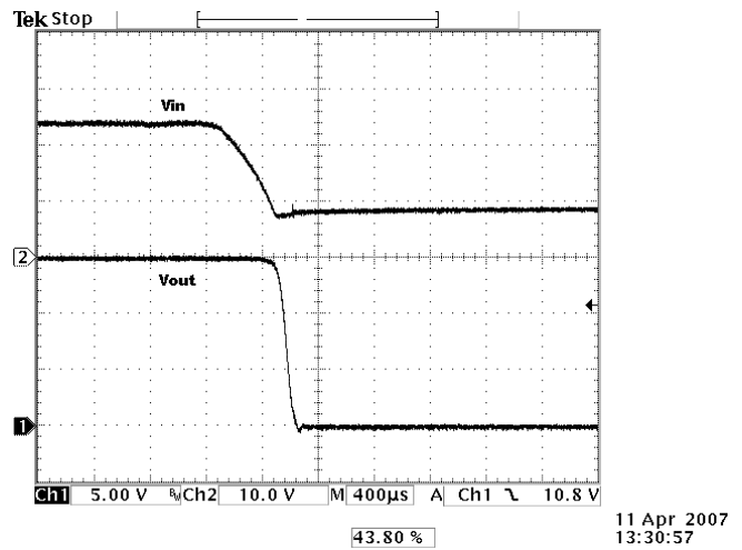
Photo 4: Normal Turn Off at 24 V Cout = 68 uF
