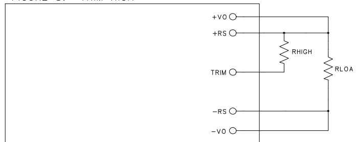
FIGURE 5: TRIM HIGH
