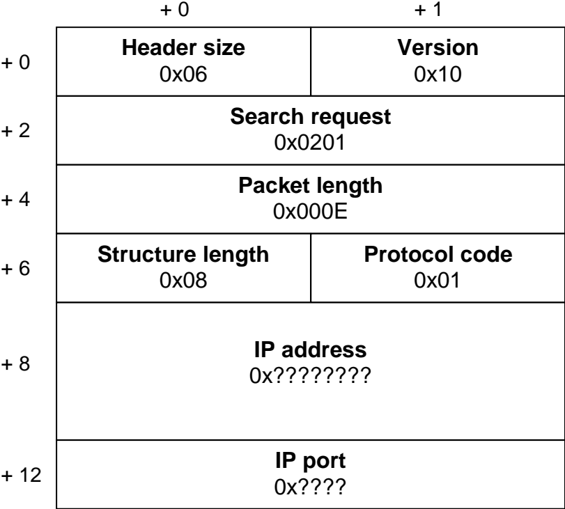
Figure 5. Structure of the Search.Req packet
