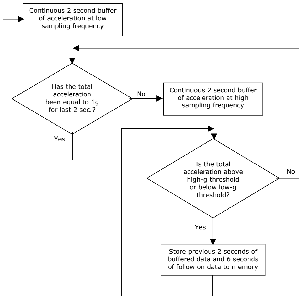
Fig. 2) Warranty protection flowchart
