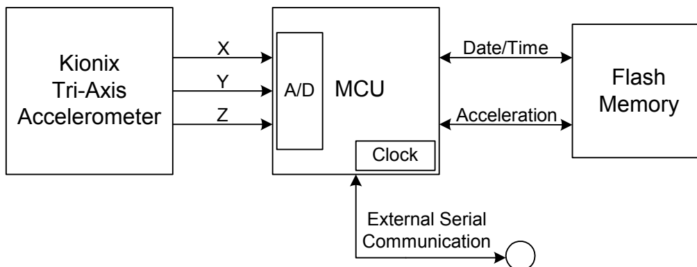
Fig. 1) Warranty Protection System Block Diagram
