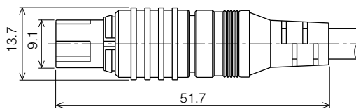
PLUG
