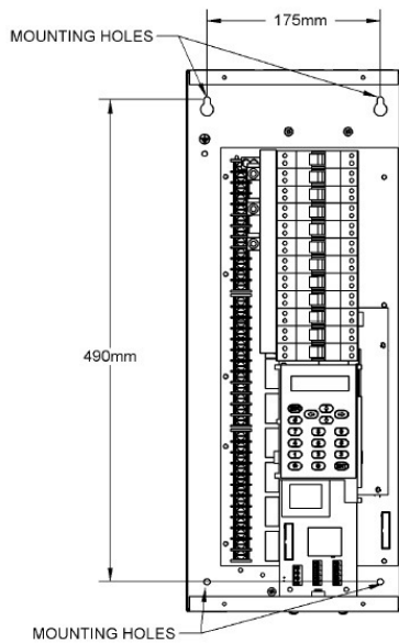
Figure 2-7: Chilli Pro 1210 HF Dimmer
