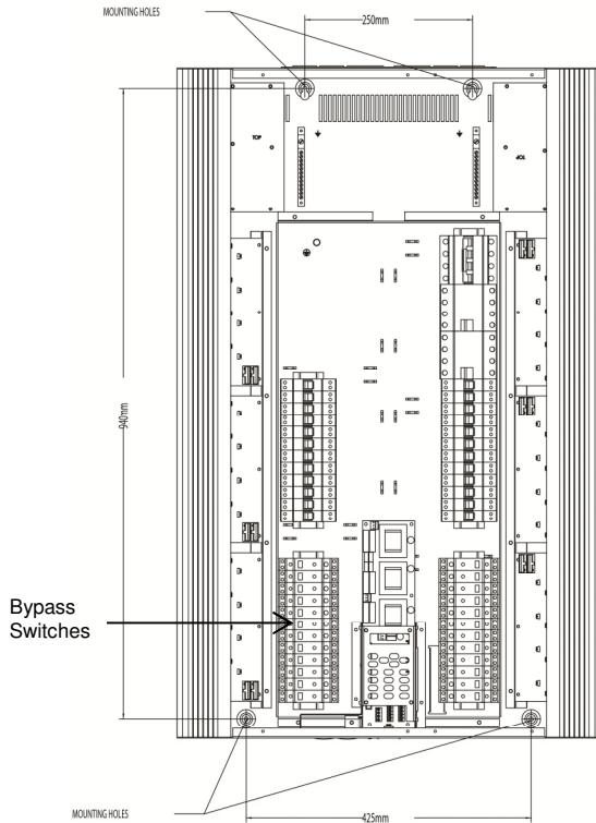
Figure 2-12: Chilli 24 Bypass Channel Dimmer
