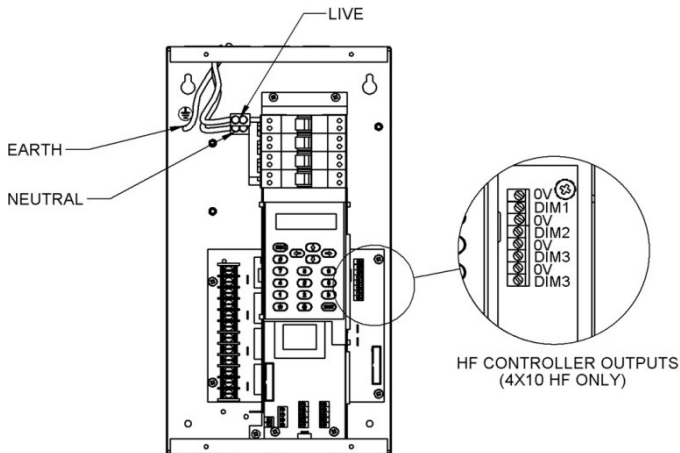
Figure 2-3: Chilli Pro 4 Channel Dimmer
