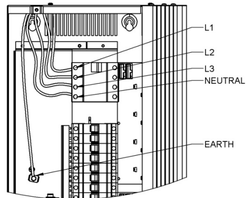
Figure 2-6: Chilli 6 or 12 Channel Dimmer (3 Phase RCD)
