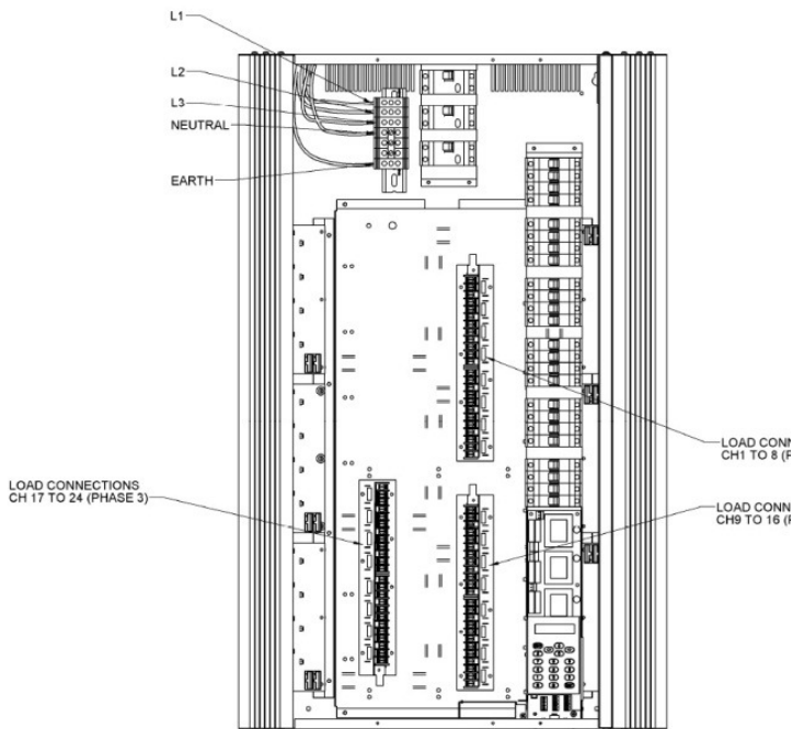
Figure 2-11: Chilli 24 Channel Dimmer
