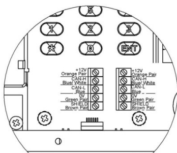
Figure 2-15: Network Connections
