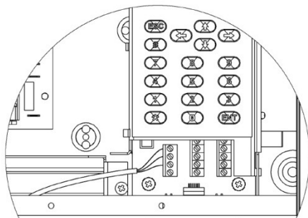
Figure 2-14: DMX Connections
