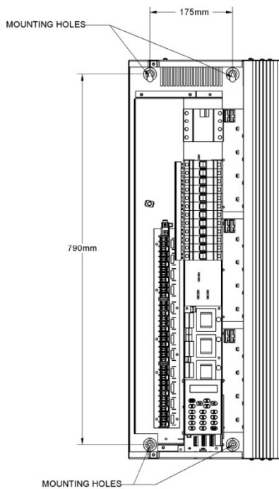
Figure 2-4: Chilli 6 or 12 Channel Dimmer
