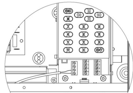
Figure 2-15: Alarm Input Connections
