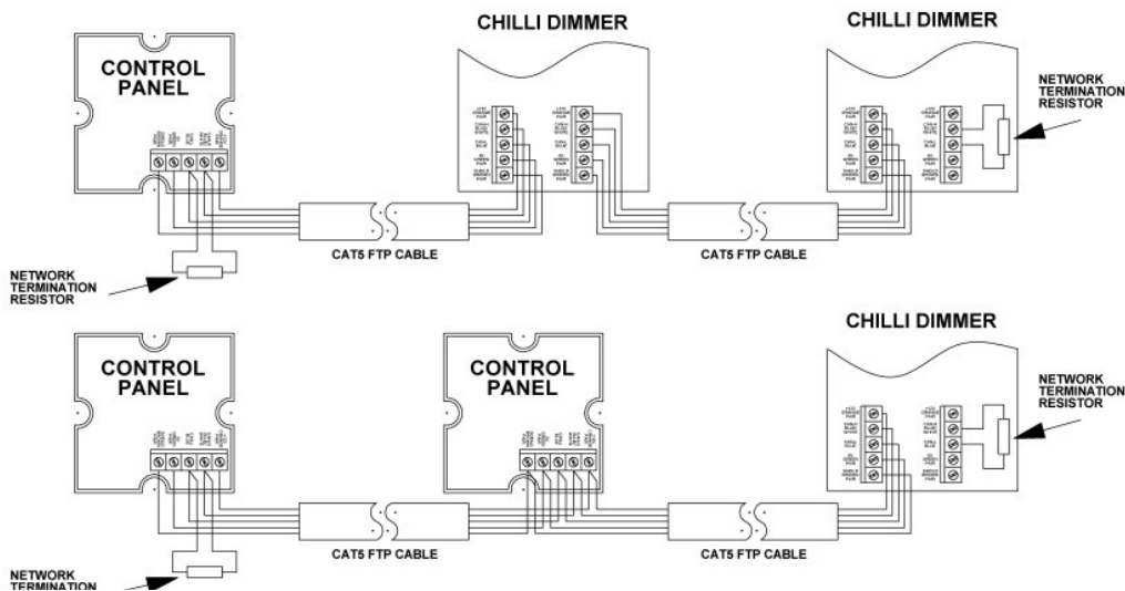
Figure 2-13: Example Chilli Net System Schematic
