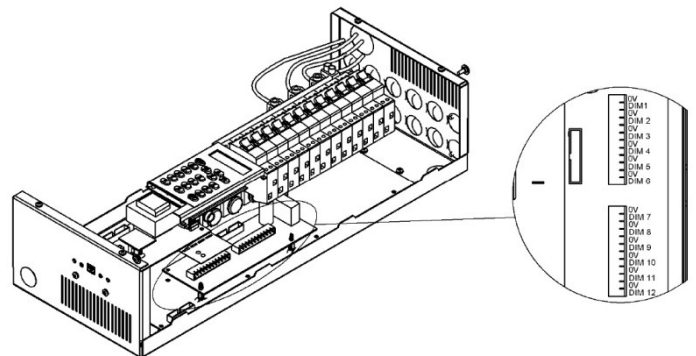
Figure 2-9: Chilli Pro 1210 HF Dimmer – HF Controller Outputs
