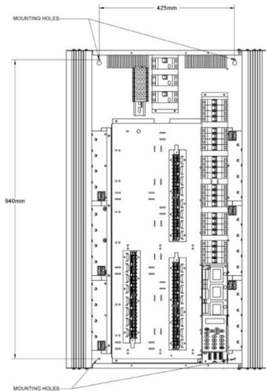
Figure 2-10: Chilli 24 Channel Dimmer
