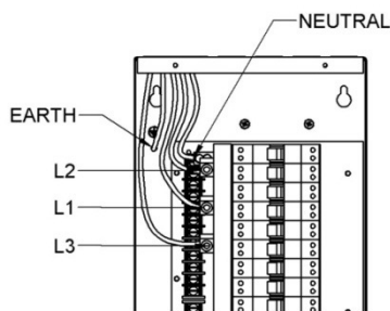
Figure 2-8: Chilli Pro 1210 HF Dimmer – Wiring
