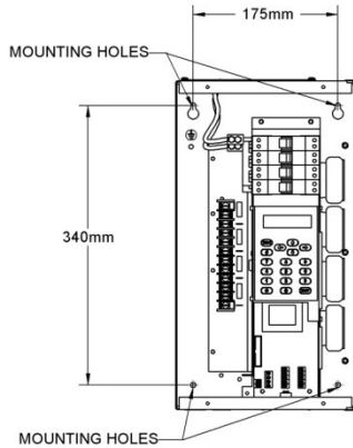
Figure 2-2: Chilli Pro 4 Channel Dimmer
