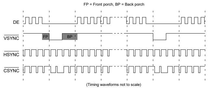
Figure 6: Output video timing (FRAME)
