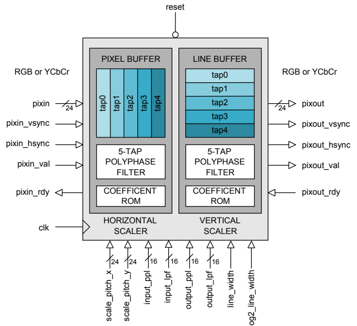
Figure 1: Video scaler architecture
