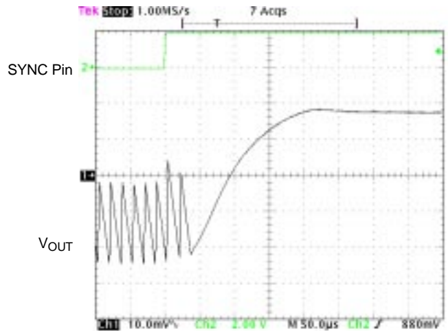
Figure 25. Pulsed Mode to PWM Mode Transition
