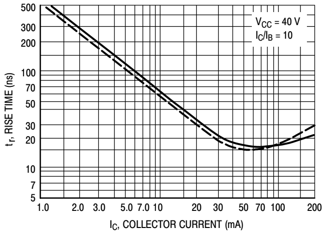
Figure 6. Rise Time
