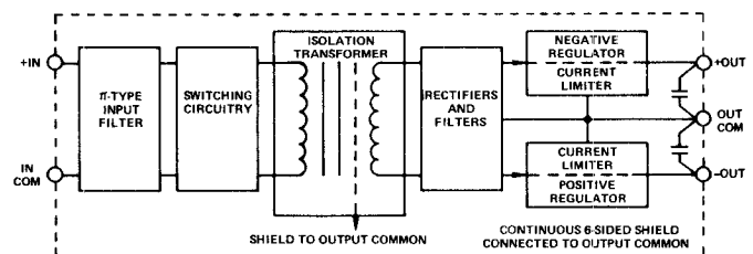
Block Diagram – Models 940, 941, 945, 951 and 953
