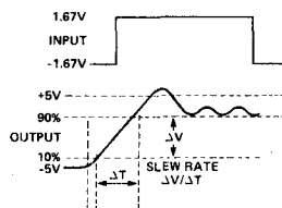
SLEW RATE
