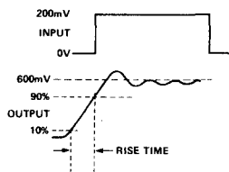
TRANSIENT RESPONSE
