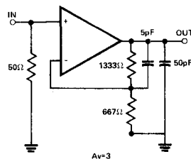
SLEW RATE AND TRANSIENT RESPONSE
