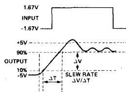
SLEW RATE
