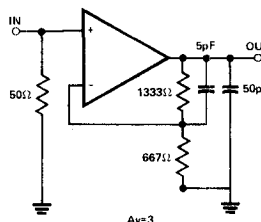
SLEW RATE AND TRANSIENT RESPONSE
