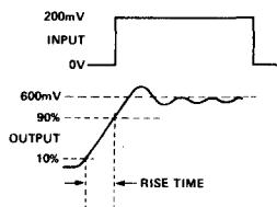
TRANSIENT RESPONSE
