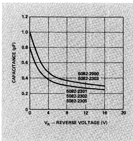
Figure 11. 5082-2300 and -2900 Series Typical Capacitance vs. Reverse Voltage.
