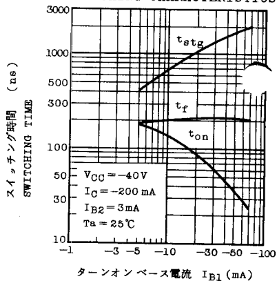
SWITCHING CHARACTERISTICS
