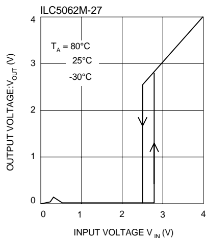
V_{OUT} vs V_{IN}
