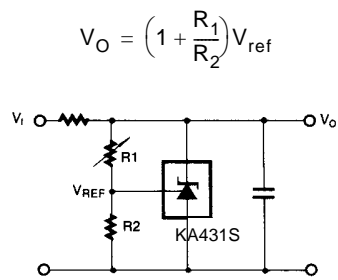
Figure 13. Shunt Regulator
