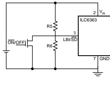
Figure 8: Shut Down Control
