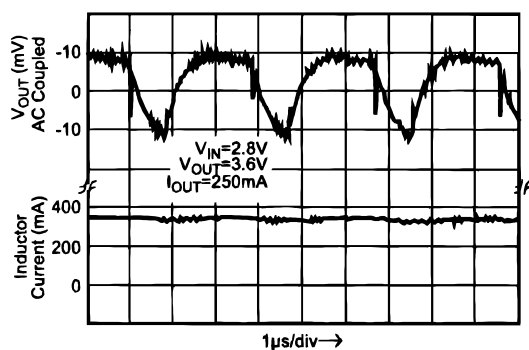
PWM Mode Load Switching Waveform
