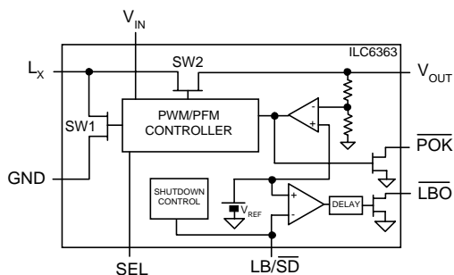
Figure 4: Simplified ILC6363 block diagram
