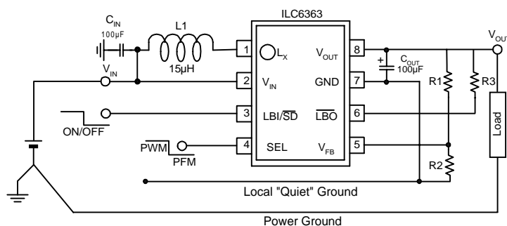
Recommended application circuit schematic for ILC6363CIR-ADJ
