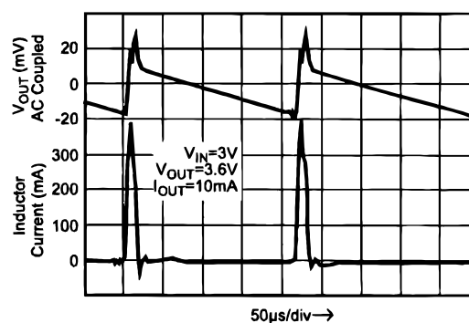
PFM Mode Load Switching Waveform
