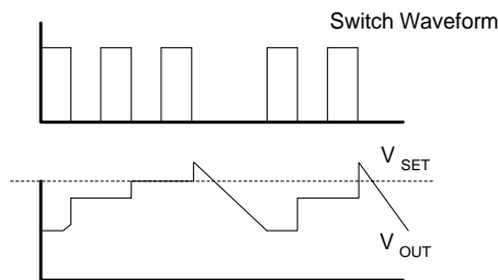
Figure 5: PFM Waveform
