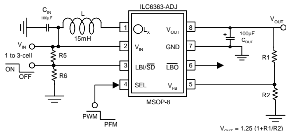
Figure 9: Adjustable Voltage Configuration
