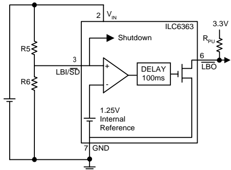
Figure 6: Low Battery Detector
