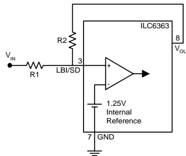
Figure 7: V_{LBI} < 1.25V
