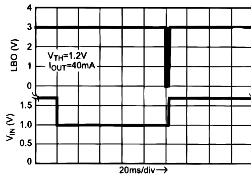
Low Battery Output ( V_{IN} < V_{TH} for Greater than 100ms) 10k \Omega pull-up resistor from LBO to 3V supply
