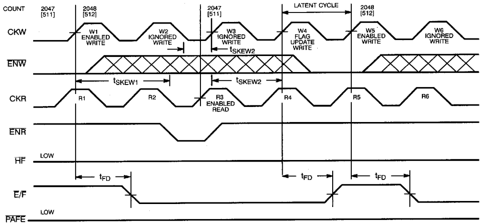
Write to Full Flag Timing Diagram with Free-Running Clocks [25, 26, 33, 40]
