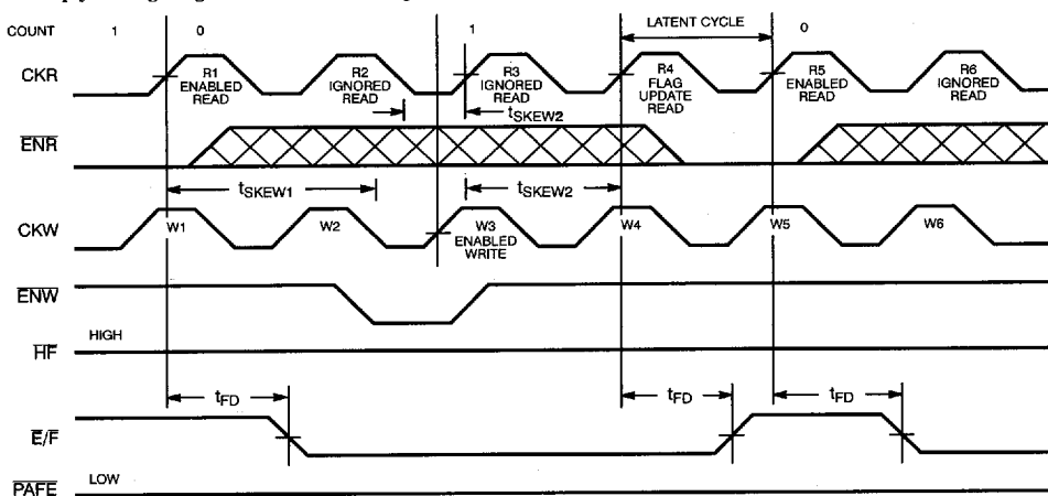
Read to Empty Timing Diagram with Free-Running Clocks [25, 26, 27, 28]
