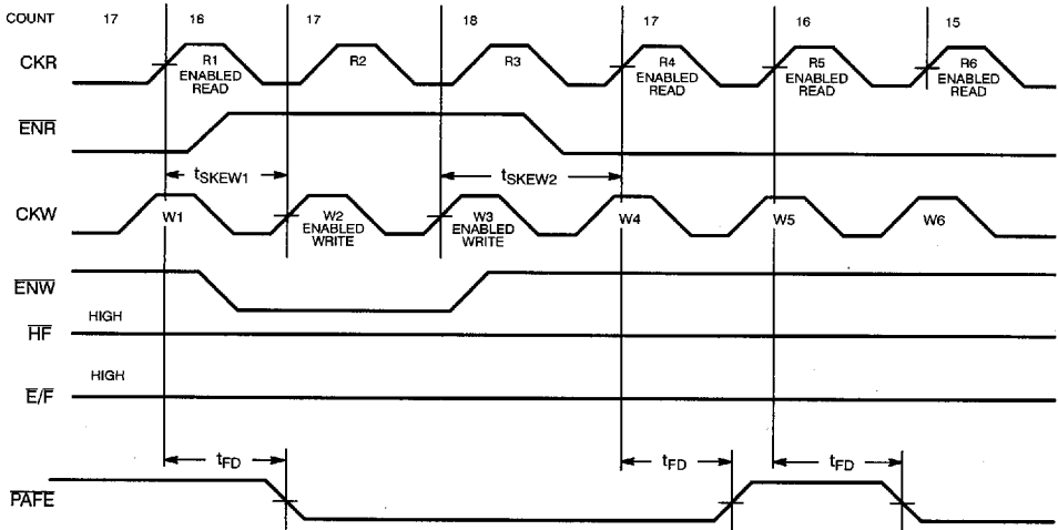
Read to Almost Empty Timing Diagram with Free-Running Clocks [25, 28, 30]
