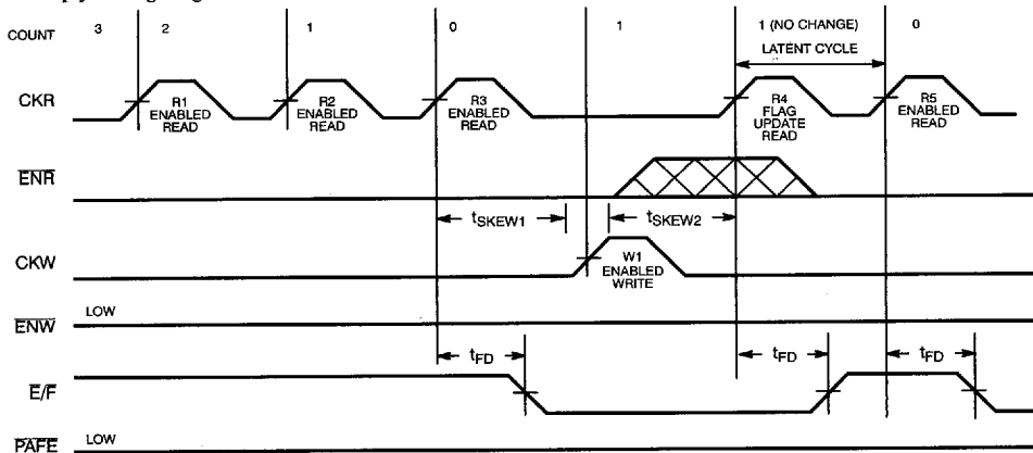
Read to Empty Timing Diagram [25, 28, 29]
