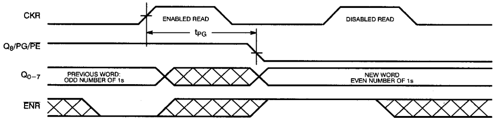
Even Parity Generation Timing Diagram [41, 43]
