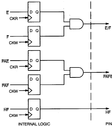
Figure 1. Flag Logic Diagram
