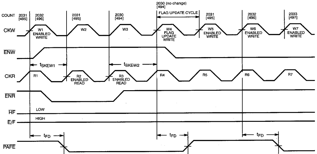
Write to Almost Full Timing Diagram with Write Flag Update Cycle and Free-Running Clocks [25, 30, 33]
