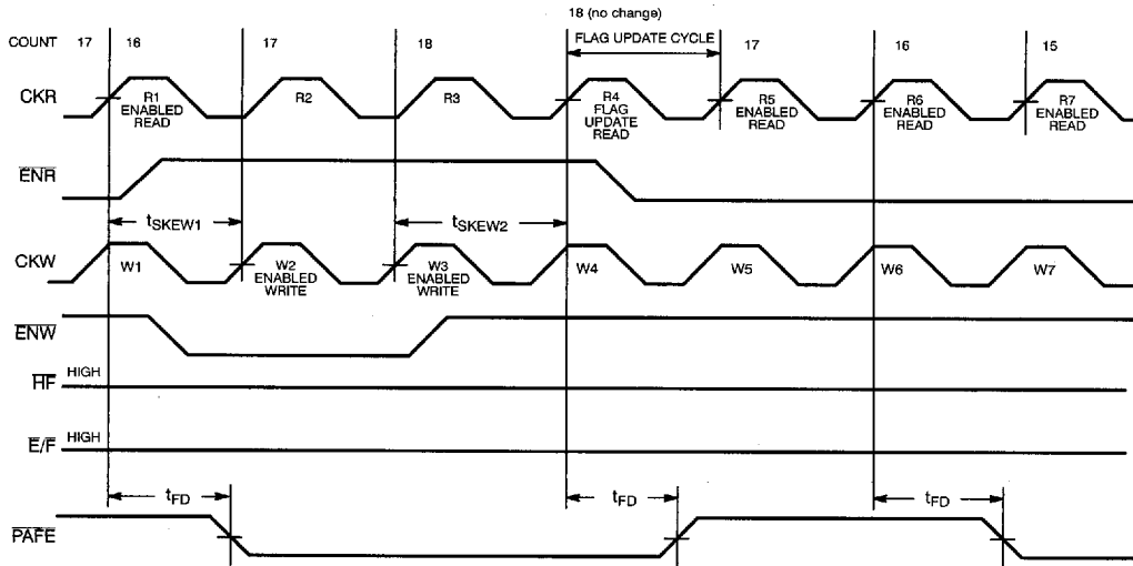
Read to Almost Empty Timing Diagram with Read Flag Update Cycle and Free-Running Clocks [25, 28, 30, 31, 32]
