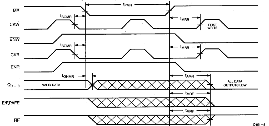
Master Reset (Default with Free-Running Clocks) Timing Diagram [21, 22, 23, 24]
