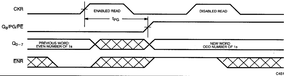
Even Parity Generation Timing Diagram [41, 43]
