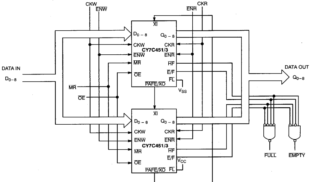
Figure 2. Depth Expansion with CY7C451/3
