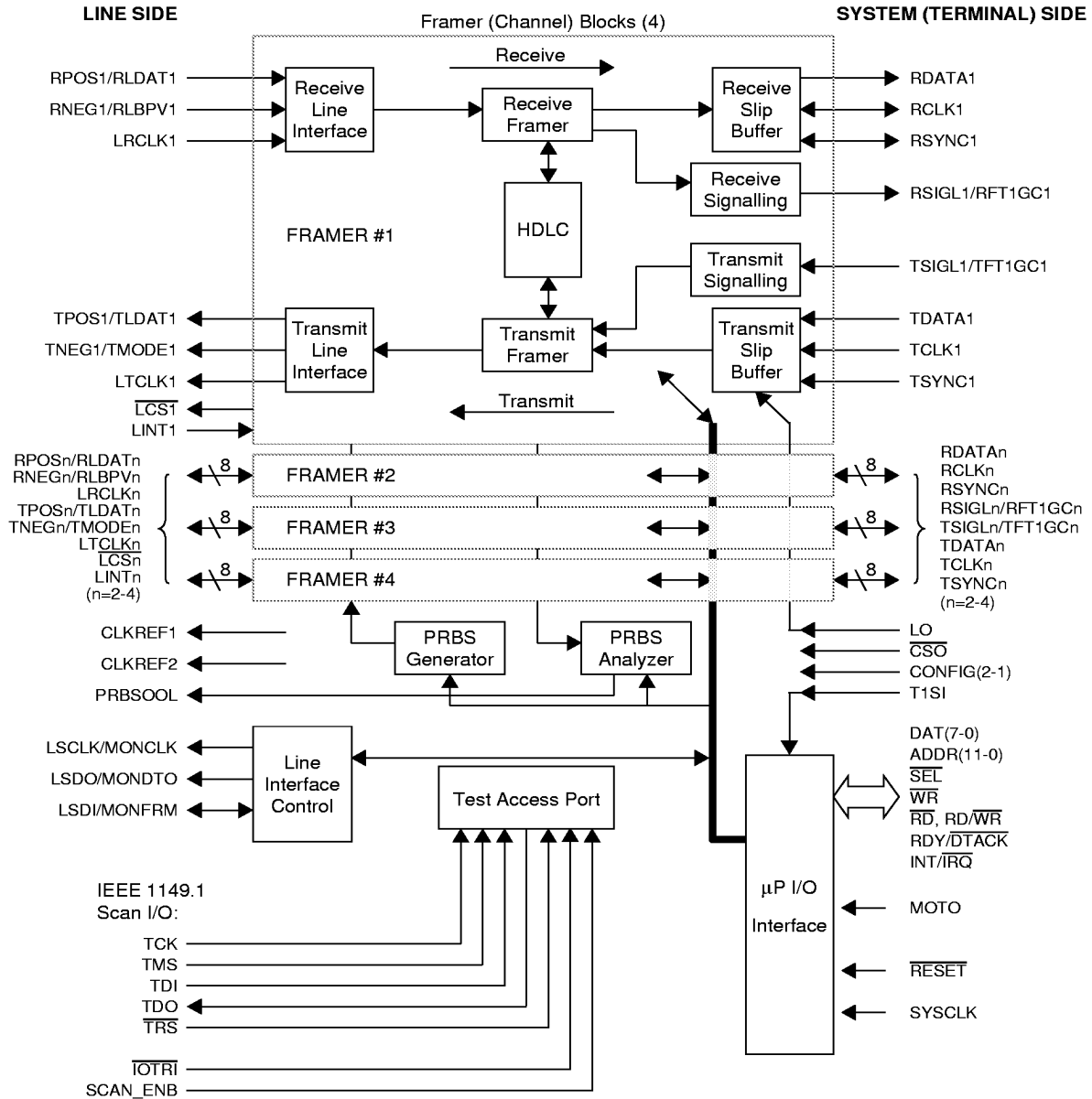
Figure 1. QT1F-Plus TXC-03103 Block Diagram
