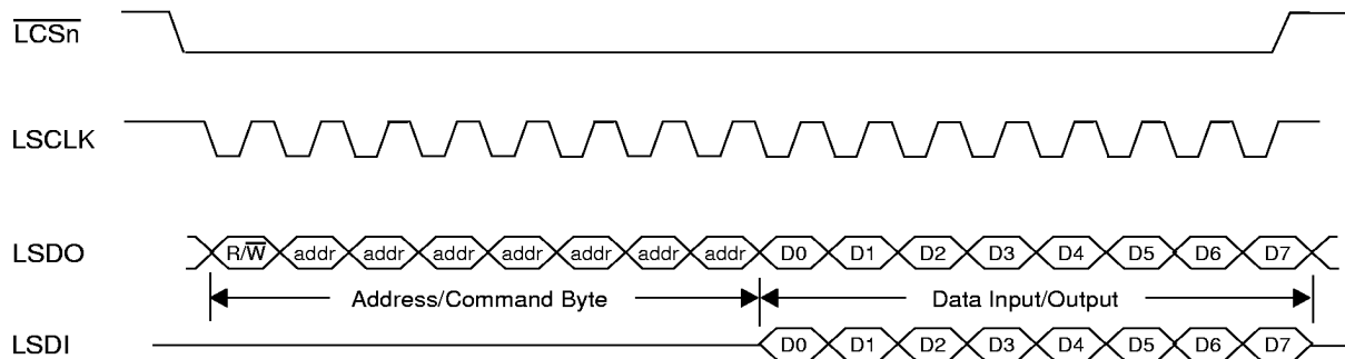
Figure 28. Transceiver Serial I/O Timing
