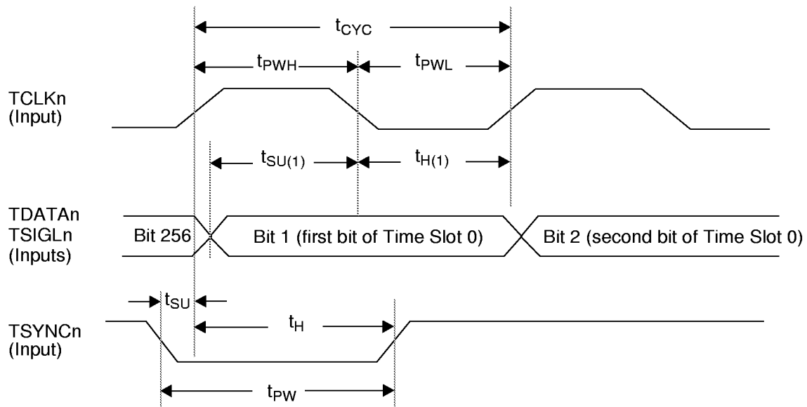
Figure 16. Transmit Highway Timing - MVIP Mode
