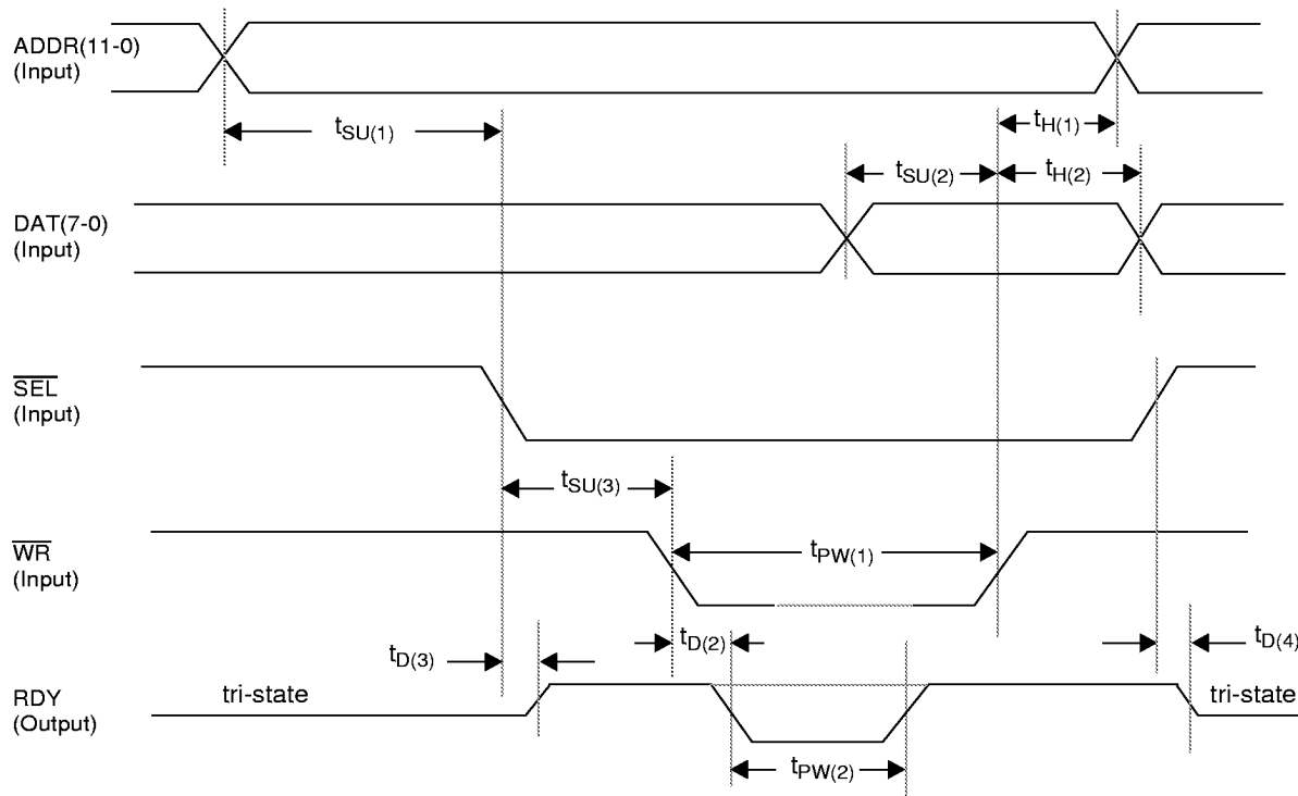
Figure 22. Intel Microprocessor Write Cycle Timing
