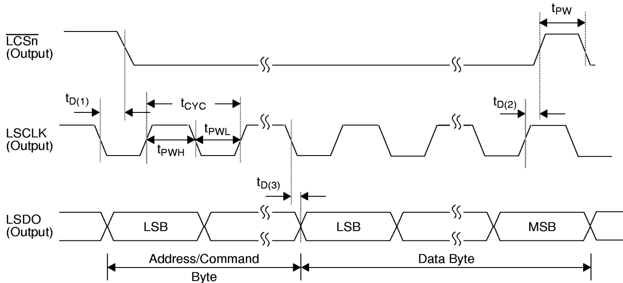
Figure 9. Serial Port Write Timing
