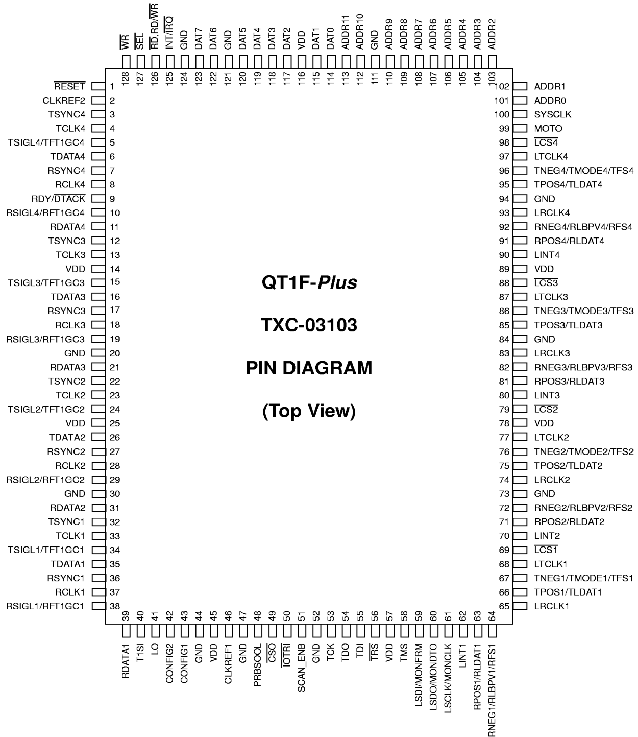
Figure 2. QT1F-Plus TXC-03103 Pin Diagram
