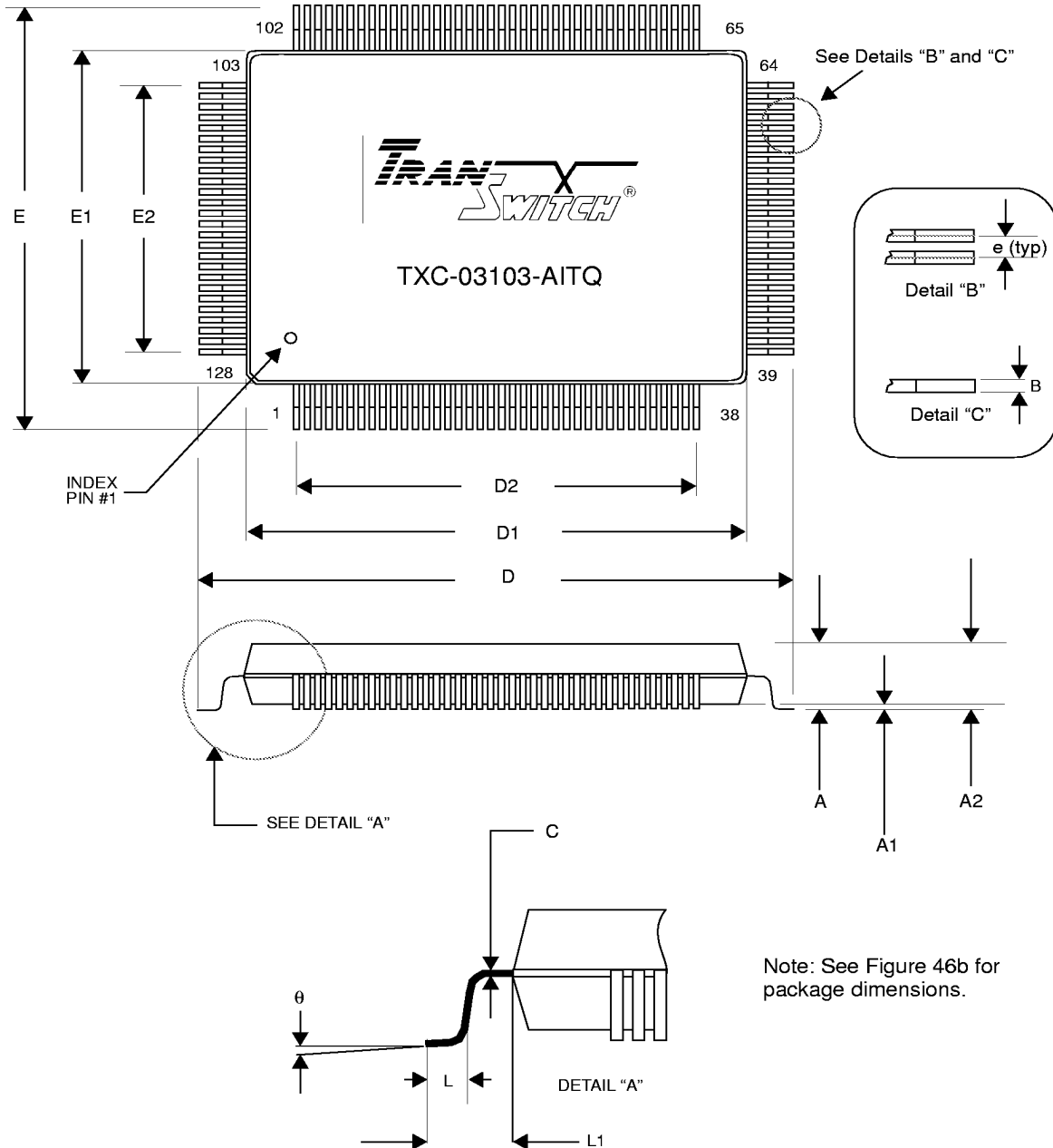
Figure 46a. QT1F-Plus TXC-03103 128-Pin Package Diagram
