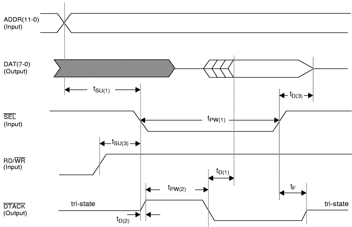
Figure 23. Motorola Microprocessor Read Cycle Timing
