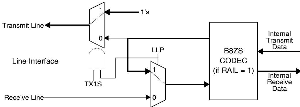
Note: Bold/dashed lines show paths used for TX1S=1 and LLP=1.
