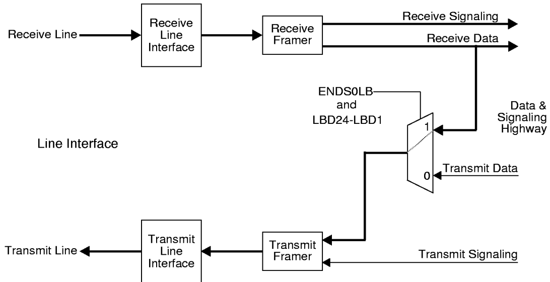
Figure 43. Payload Remote Loopback
