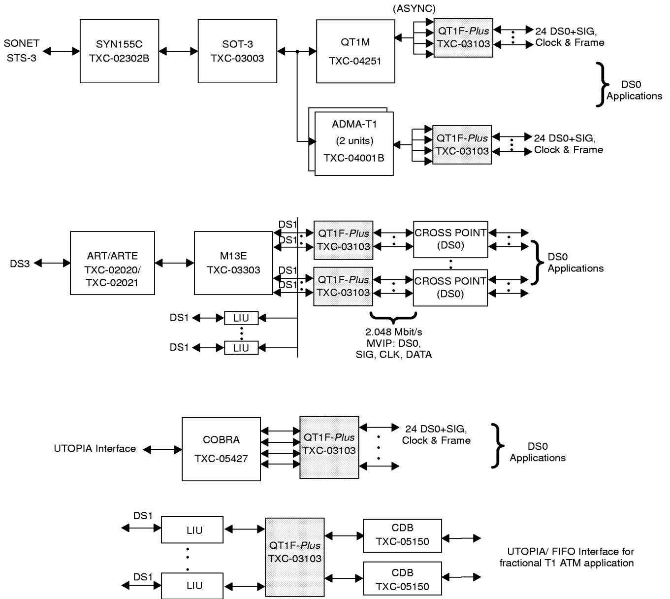
Figure 45. Some QT1F-Plus TXC-03103 Applications
