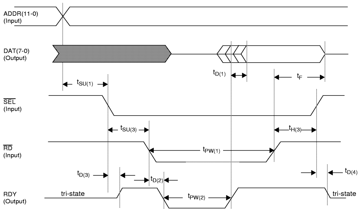
Figure 21. Intel Microprocessor Read Cycle Timing
