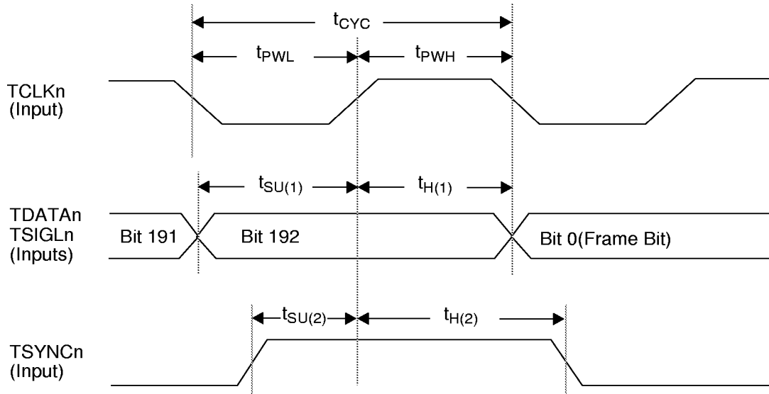
Figure 14. Transmit Highway Timing - Transmission Mode
