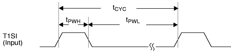
Figure 19. Shadow Register Timing
