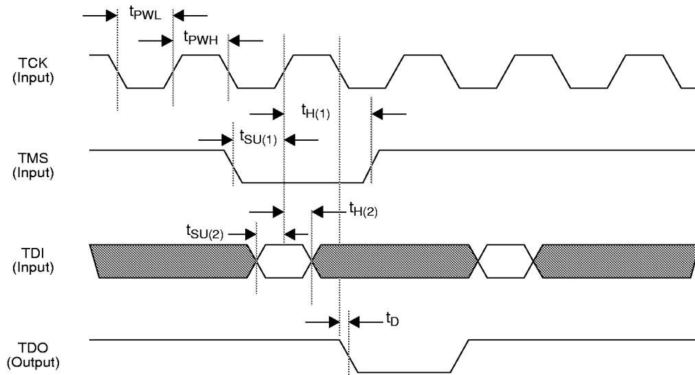
Figure 20. Boundary Scan Timing
