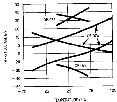
Offset Voltage Drift With Temperature Of Representative Units
