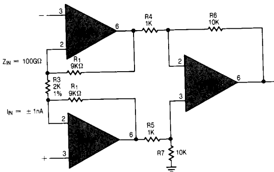
Instrumentation Amplifier
