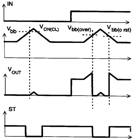
Figure 7a: Overvoltage:
