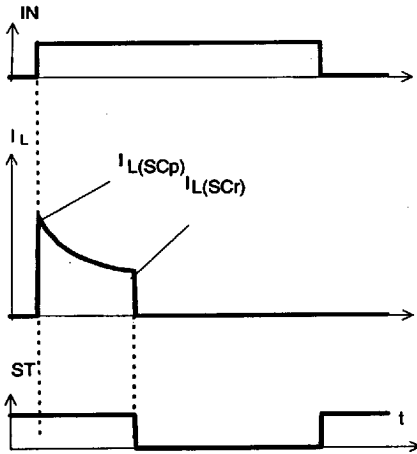
Figure 3b: Turn on into overload,
