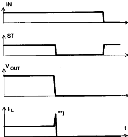
Figure 3c: Short circuit while on:
