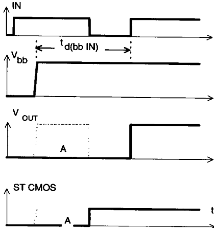
Figure 1a: V_{bb} turn on:
