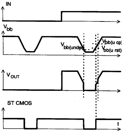
Figure 6a: Undervoltage:
