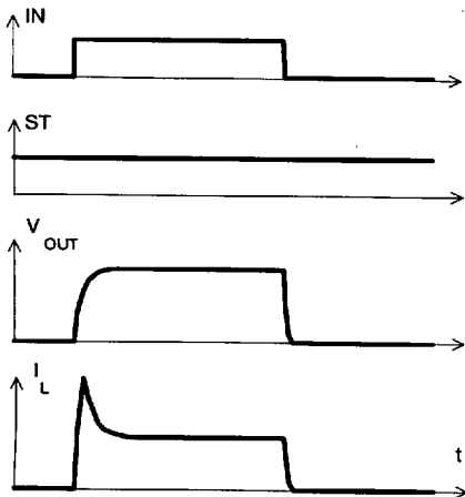
Figure 2a: Switching a lamp,
