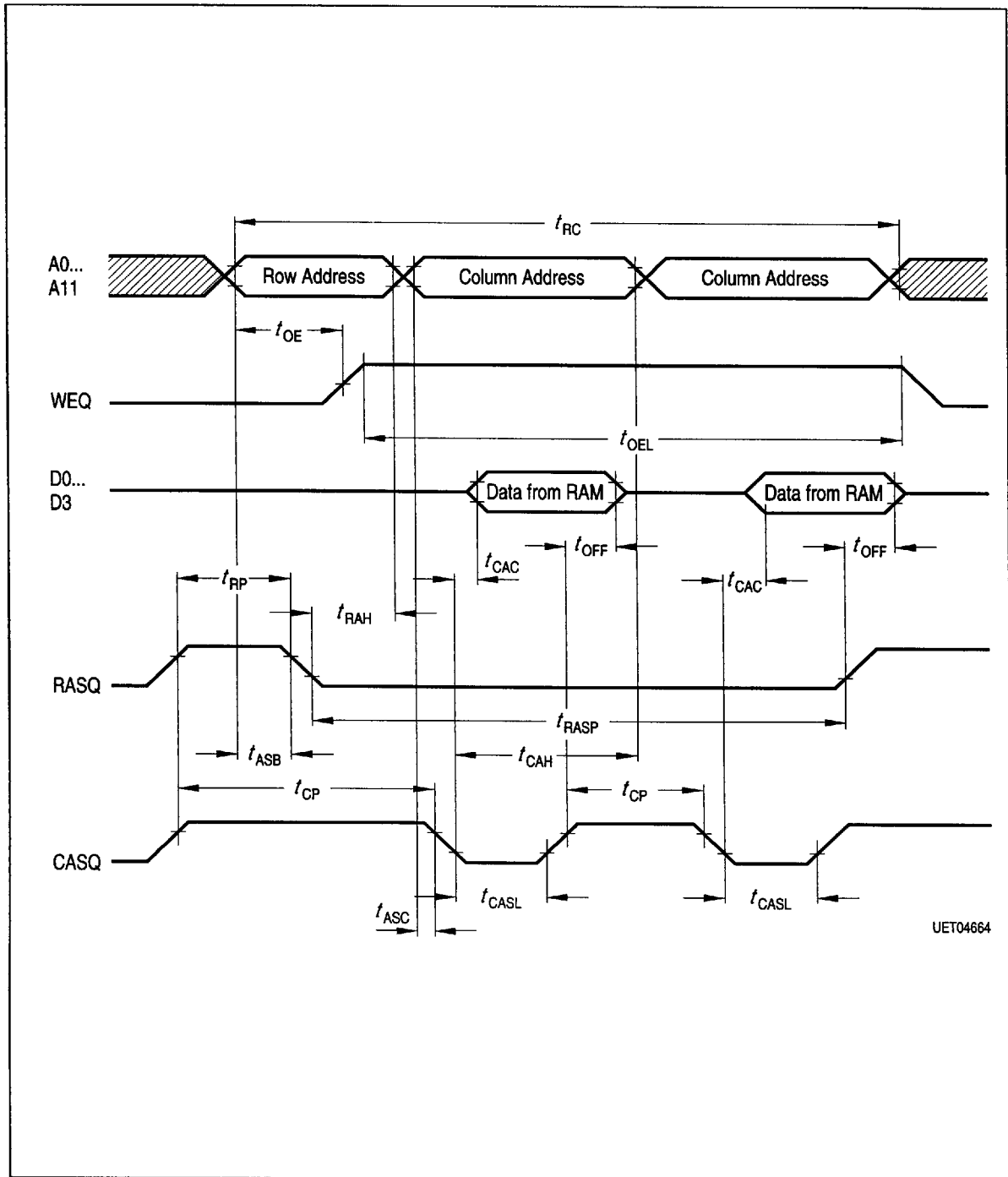
Timing Diagram 4b DRAM-Page Mode Read Cycle
