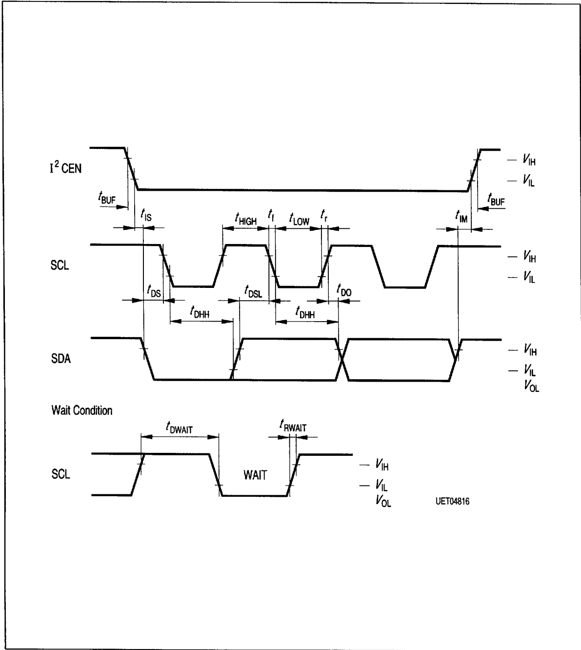
Timing Diagram 3b M3L-Bus Mode
