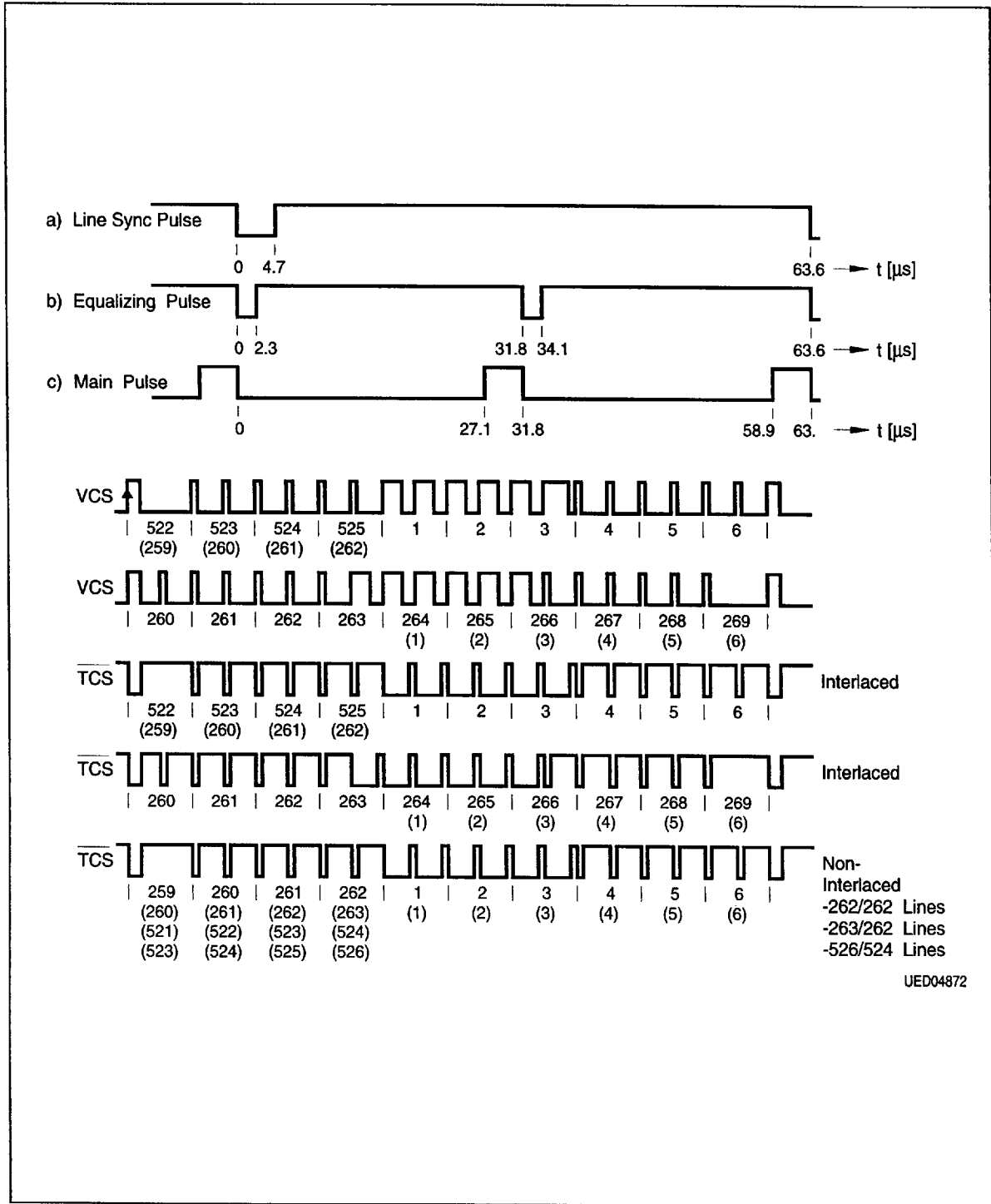
Timing Diagram 5b VCS and TCS in NTSC Freerun Mode
