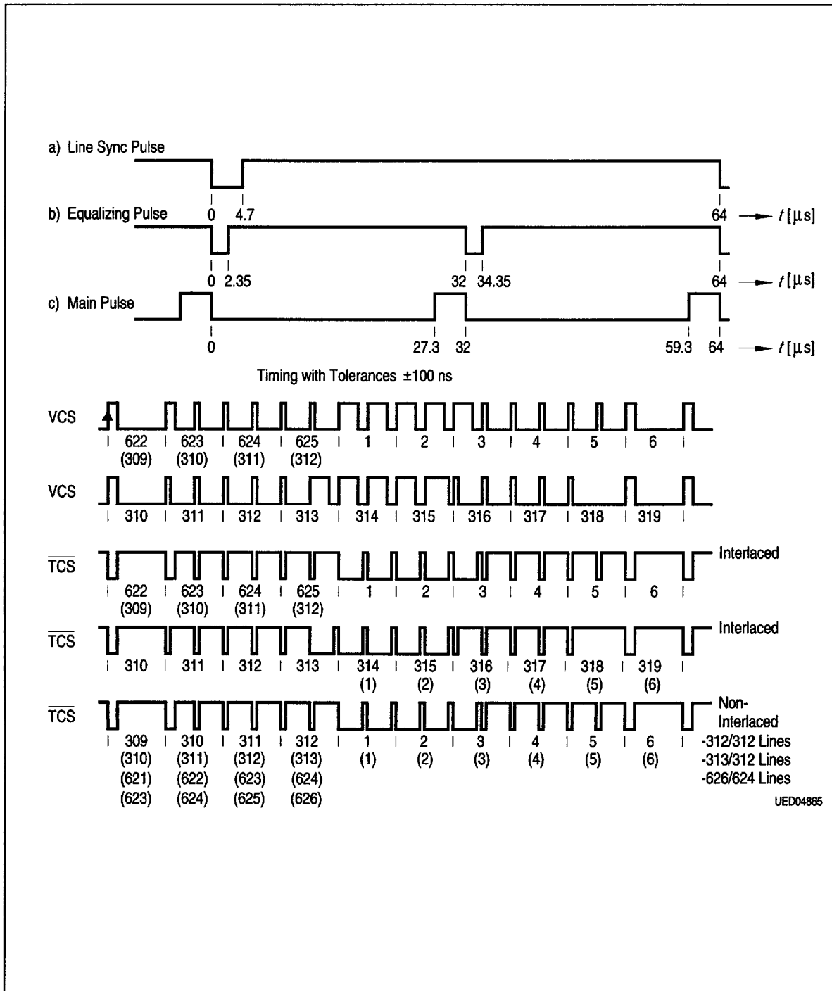
Timing Diagram 5a VCS and TCS in PAL Freerun Mode
