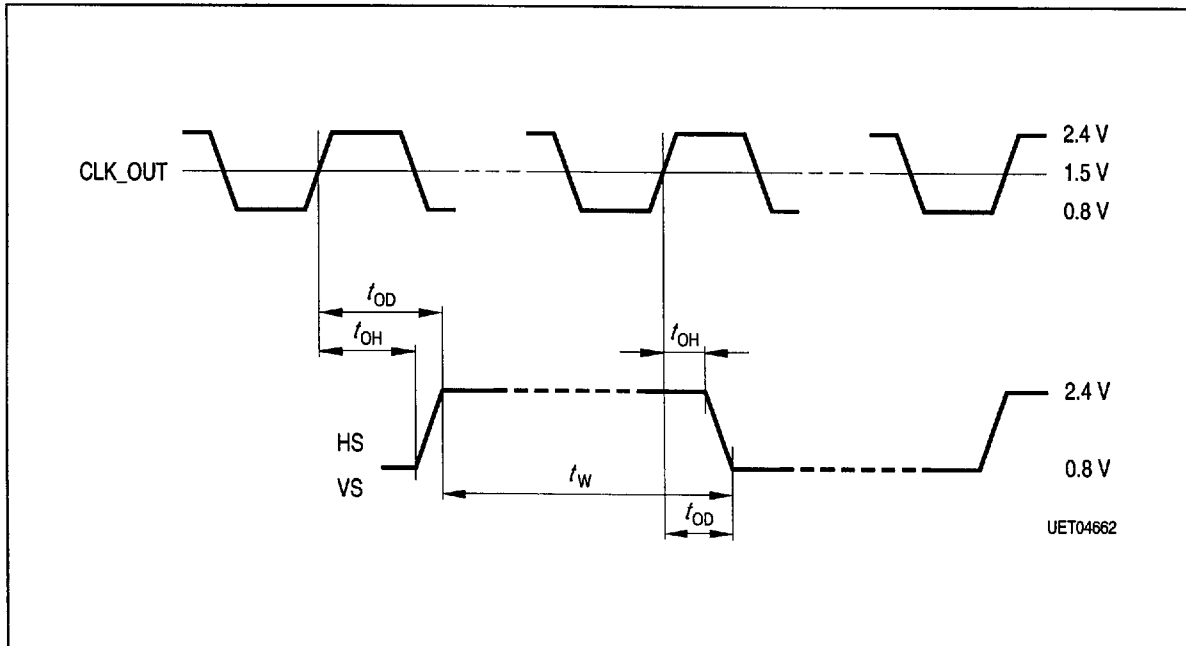
Timing Diagram 2
