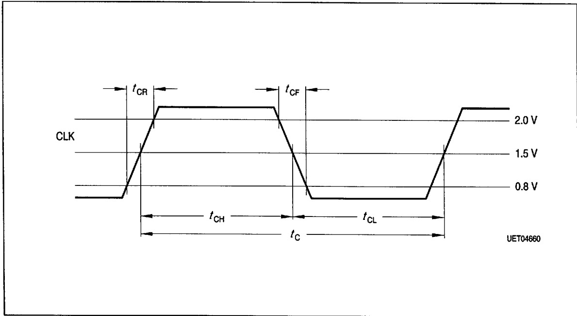
Timing Diagram 1
