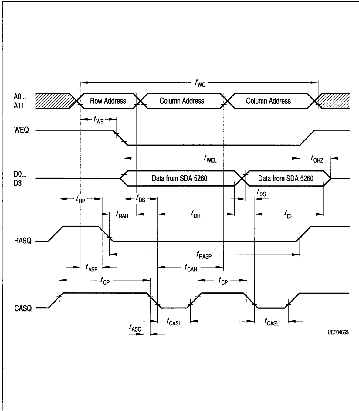
Timing Diagram 4a DRAM-Page Mode Write Cycle
