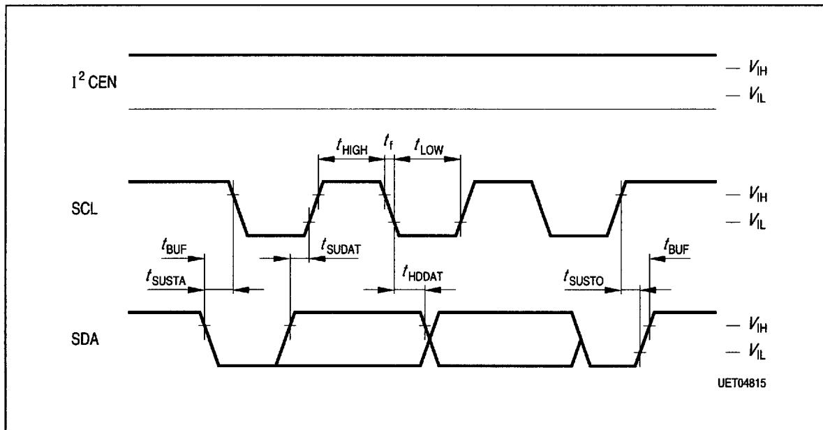
Timing Diagram 3a I 2 C-Bus Mode
