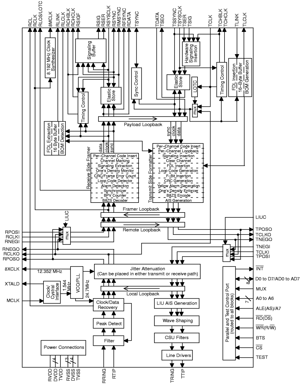
DS2152 ENHANCED T1 SINGLE-CHIP TRANSCIEVER Figure 1-1
