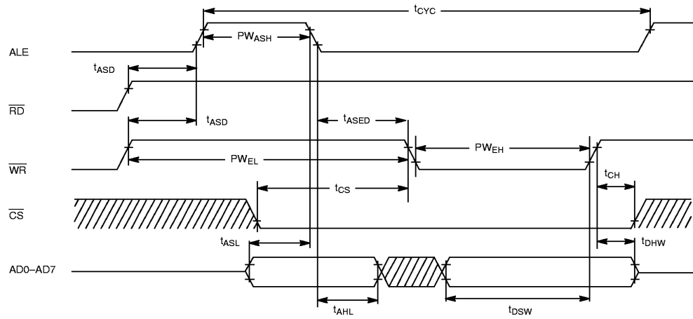
INTEL BUS WRITE AC TIMING (BTS=0/MUX=1) Figure 16-2
