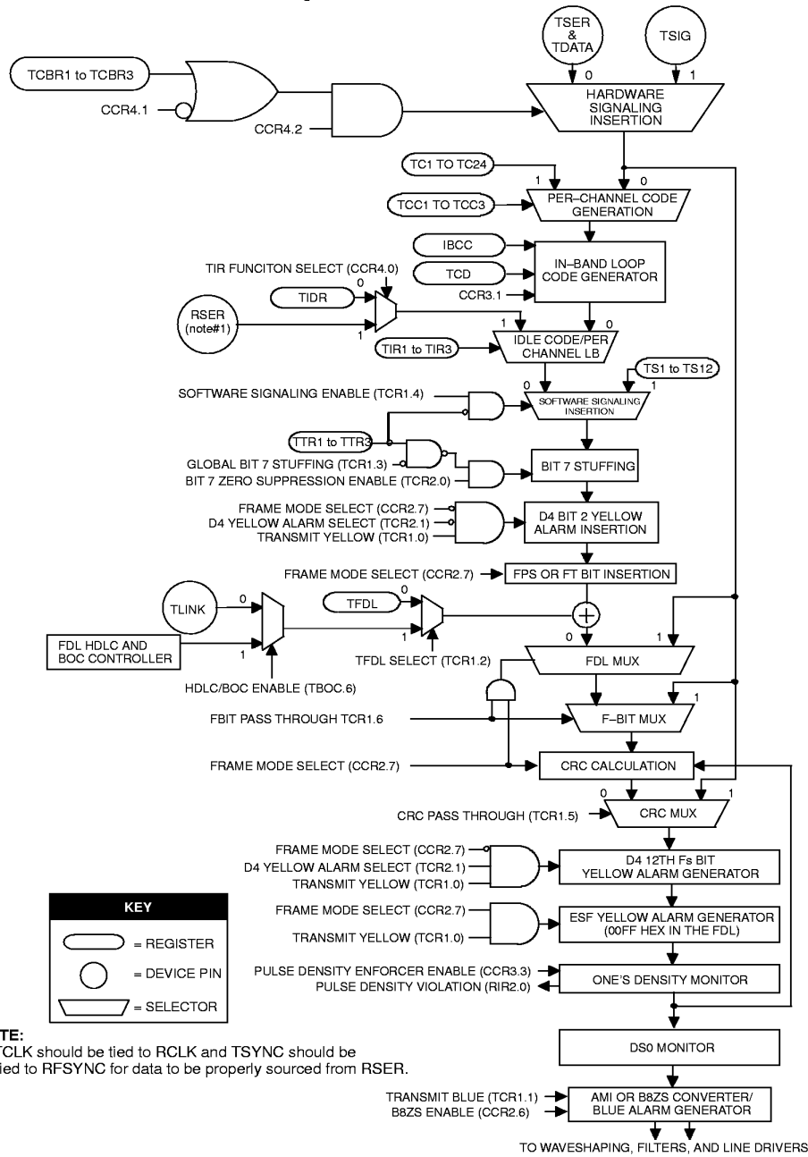
DS2152 TRANSMIT DATA FLOW Figure 15-11
