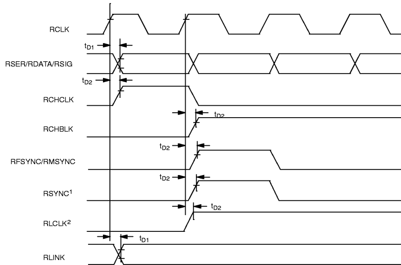
RECEIVE SIDE AC TIMING Figure 16-4
