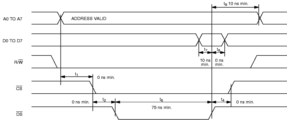
MOTOROLA BUS WRITE AC TIMING (BTS=1/MUX=0) Figure 16-13
