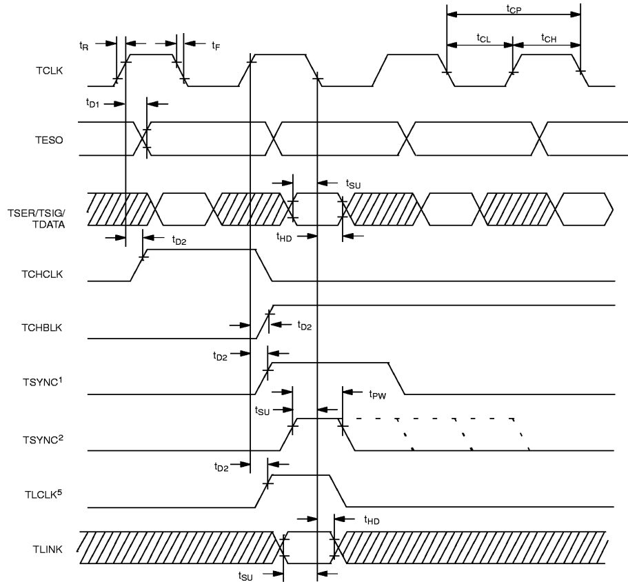
TRANSMIT SIDE AC TIMING Figure 16-7
