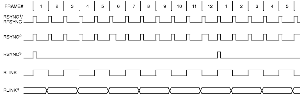
RECEIVE SIDE D4 TIMING Figure 15-1
