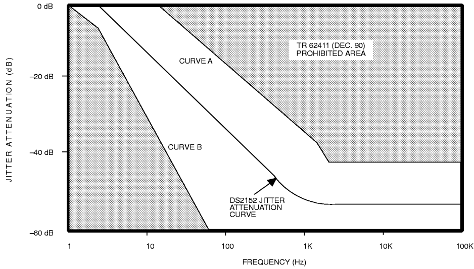
DS2152 JITTER ATTENUATION Figure 14-4
