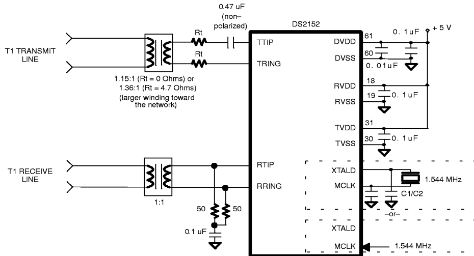
DS2152 EXTERNAL ANALOG CONNECTIONS Figure 14-1
