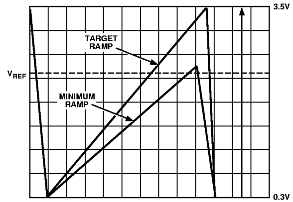
Figure 15. Current Ramp
