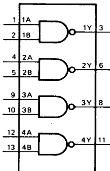
Fig. 1 Logic Symbol
