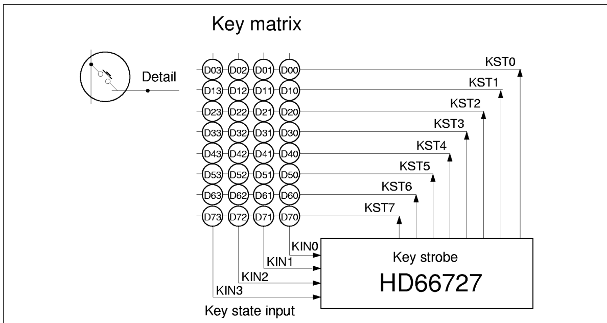
Figure 25 Key Scan Configuration
