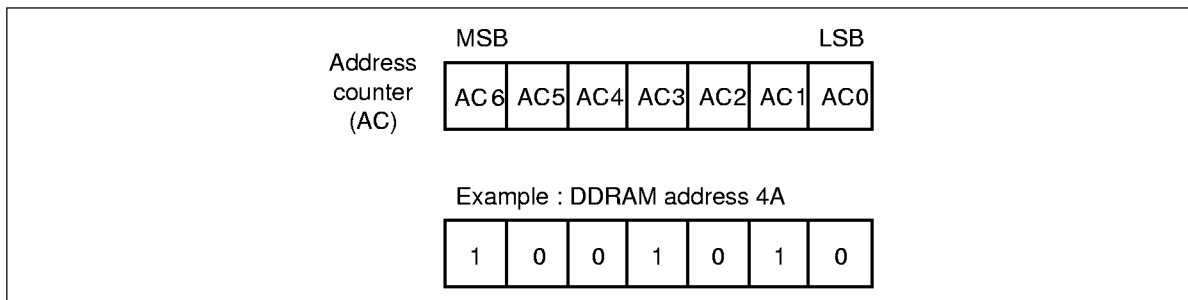
Figure 2 Address Counter and Sample DDRAM Address Setting
