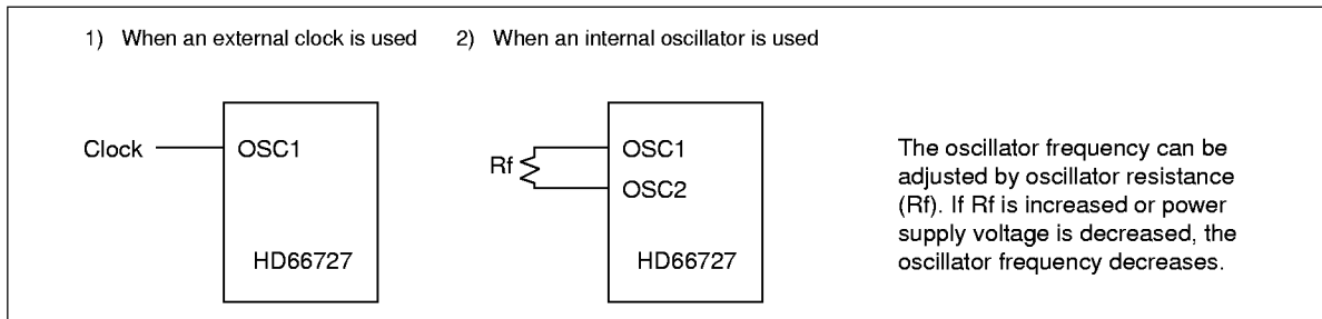
Figure 31 Oscillator Circuit
