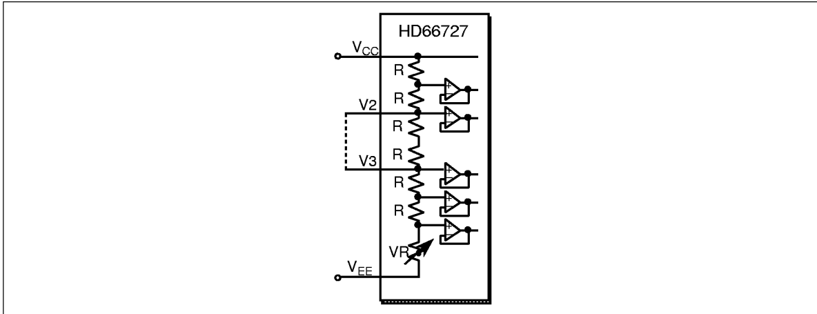
Figure 16 Contrast Adjuster
