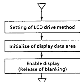
Figure 3-15. Initial Setting of LCD Driver
