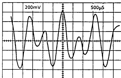
Figure 3-26. Dual tone waveform
