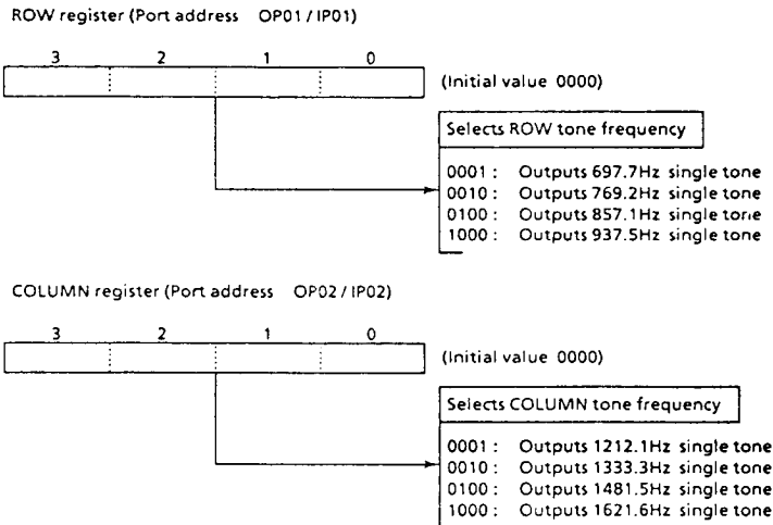
Figure 3-23. ROW, COLUMN Register
