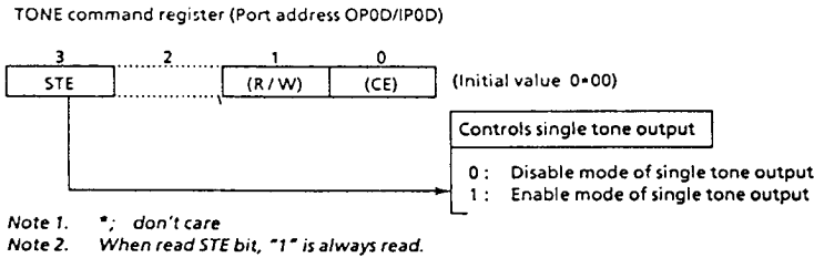
Figure 3-22. TONE command register
