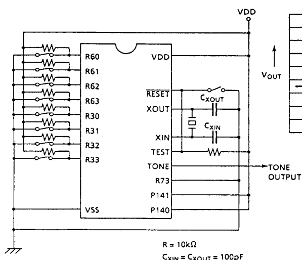
Figure 3-24. Tone test circuit
