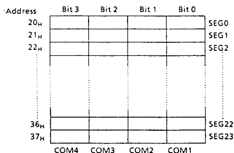
Figure 3-14. Display Data Area and SEG/COM
