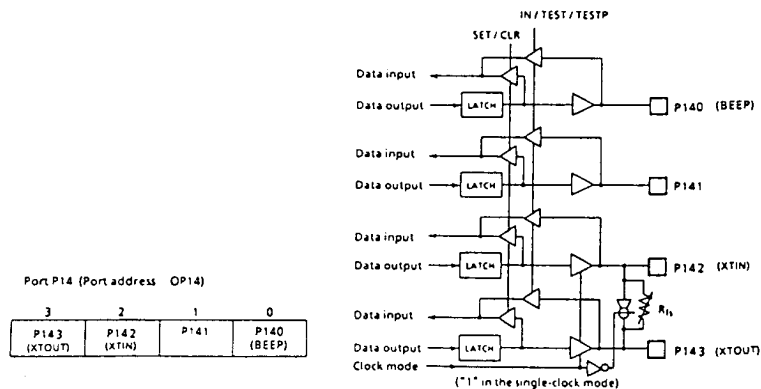
Figure 3-3. Port P14
