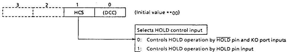
Figure 4-2. HOLD control input select command register
