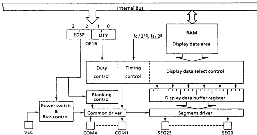
Figure 3-11. Configuration of LCD Driver
