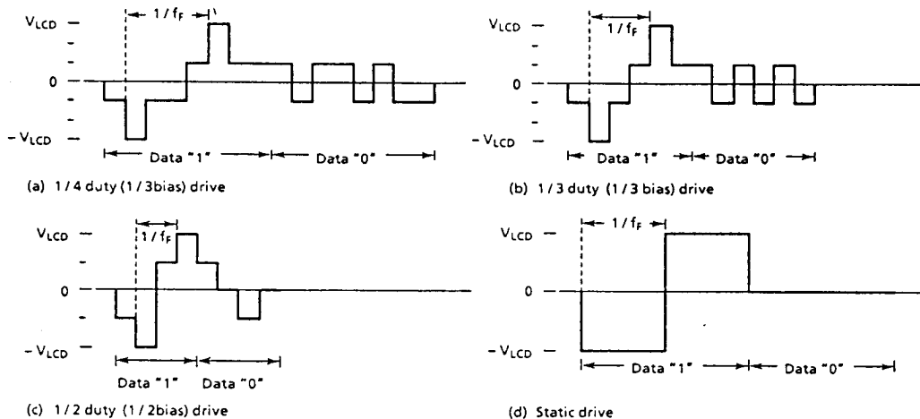
Figure 3-13. Driving Waveform for LCD (Voltage between COM-SEG)
