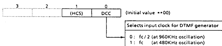
Figure 3-20. DTMF Input Clock Control Command Register
