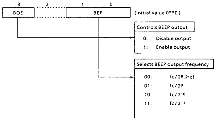
Figure 3-28. BEEP Output Control Command Register
