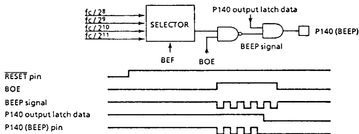
Figure 3-27. BEEP Output Circuit Configuration and Timing Chart
