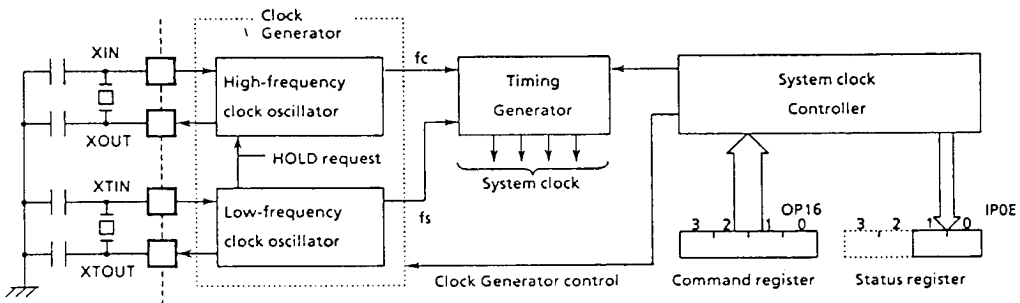
Figure 3-4. System Clock Controller
