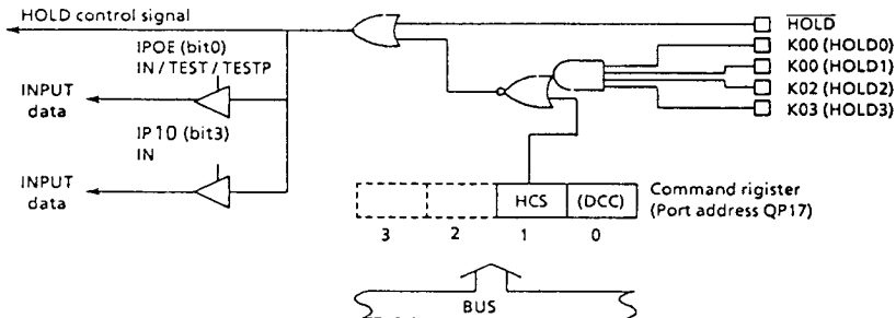
Figure 4-1. Configuration of HOLD control circuit
