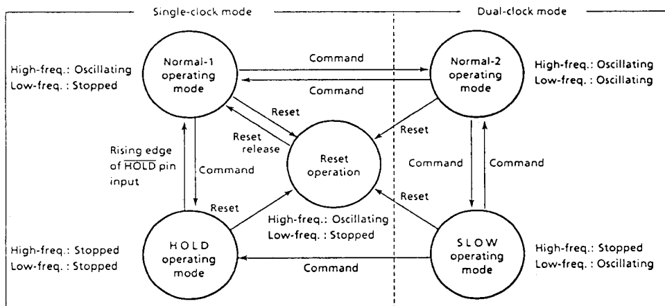
Figure 3-5. Operating Mode Transition Diagram
