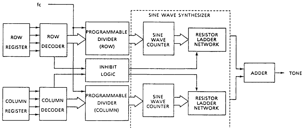
Figure 3-21. Configuration of DTMF Generator
