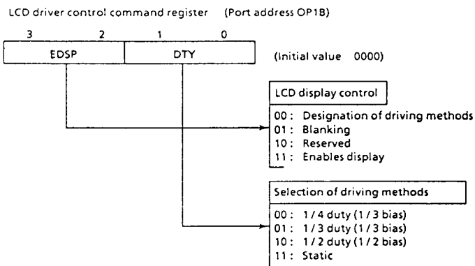
Figure 3-12. LCD Driver Control Command Register
