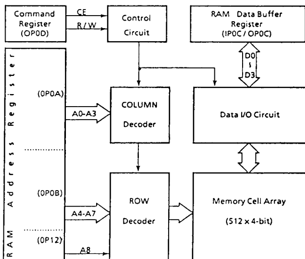
Figure 2-1. RAM. Block Diagram
