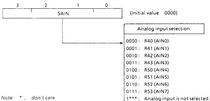
Figure 3-22. Analog input selector
