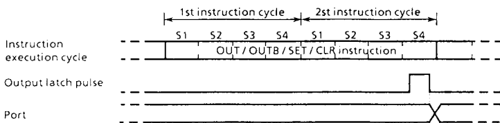
Figure 3-2. Output Timing
