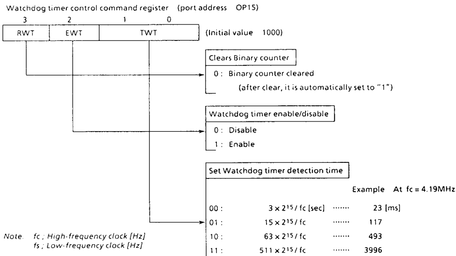
Figure3-36. Watchdog Timer Control Command Register
