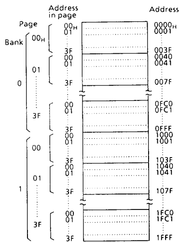
Figure 2-2. Configuration of Program Memory
