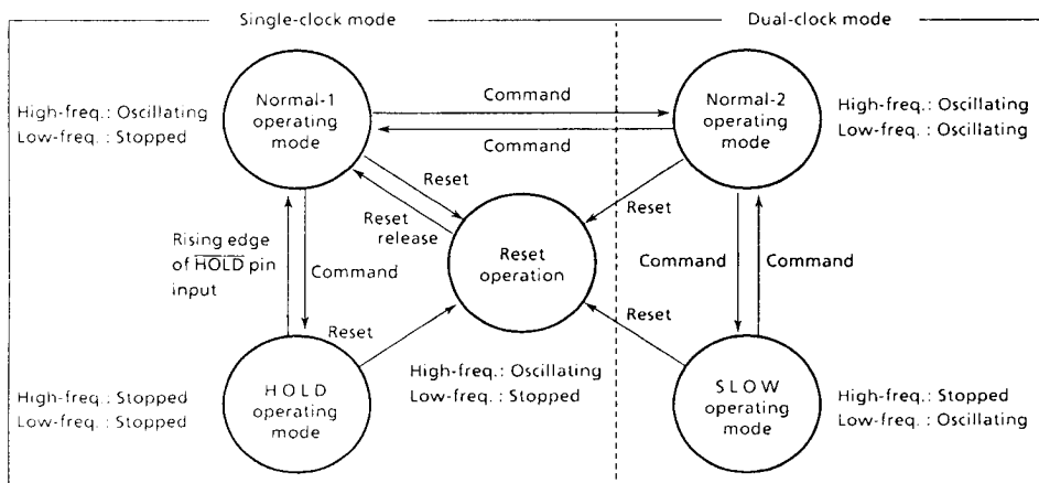
Figure 2-15. Operating Mode Transition Diagram
