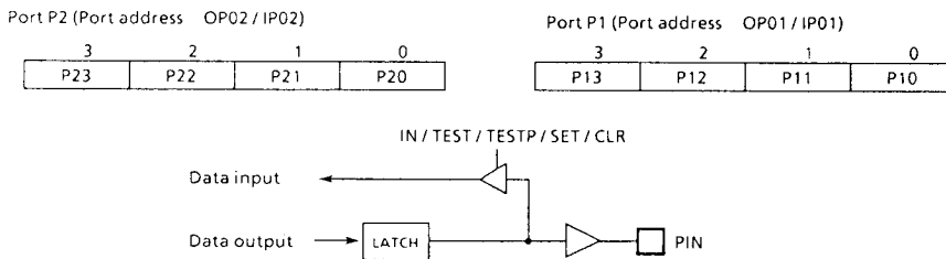
Figure 3-5. Ports P1, P2
