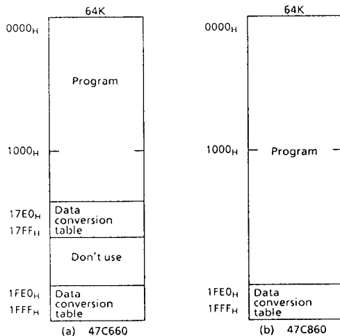
Figure 1. Program area
