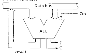
Figure 2-11. ALU
