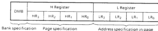
Figure 2-4. Configuration of H, L registers and DMB
