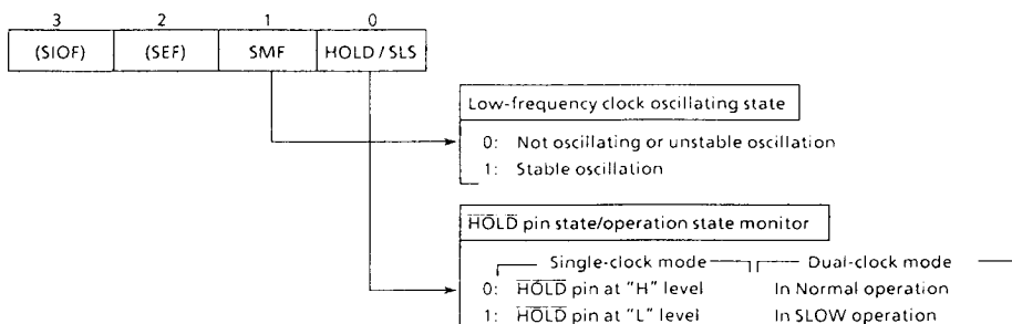
Figure 2-16. System Clock Control Command Register/Status Register
