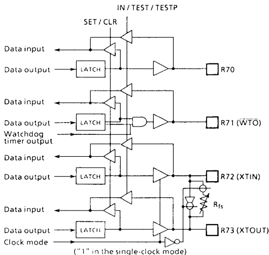
Figure 3-8. Port R7
