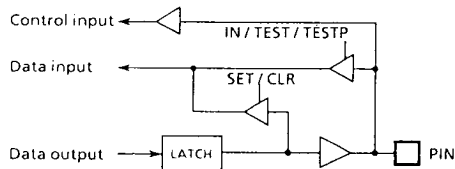
Figure 3-9. Port R8
