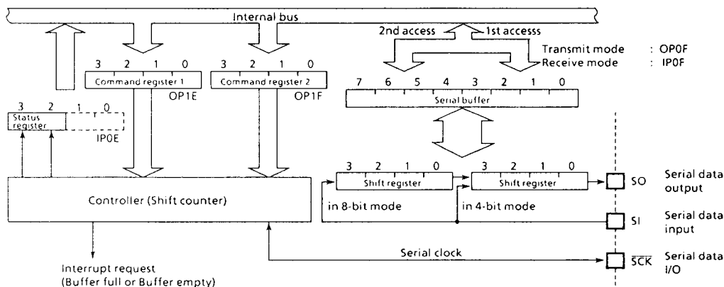
Figure 3-29. Configuration of Serial Interface
