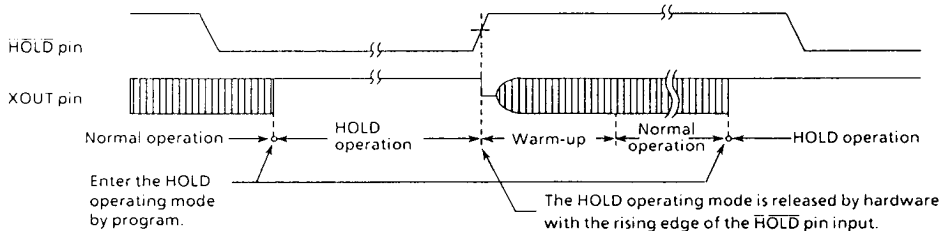
Figure 5-3. Edge-sensitive Release Mode
