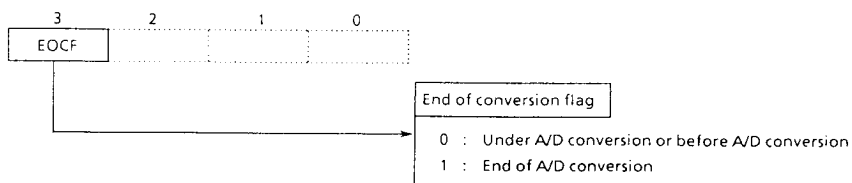
Figure 3-25. A/D converter status register
