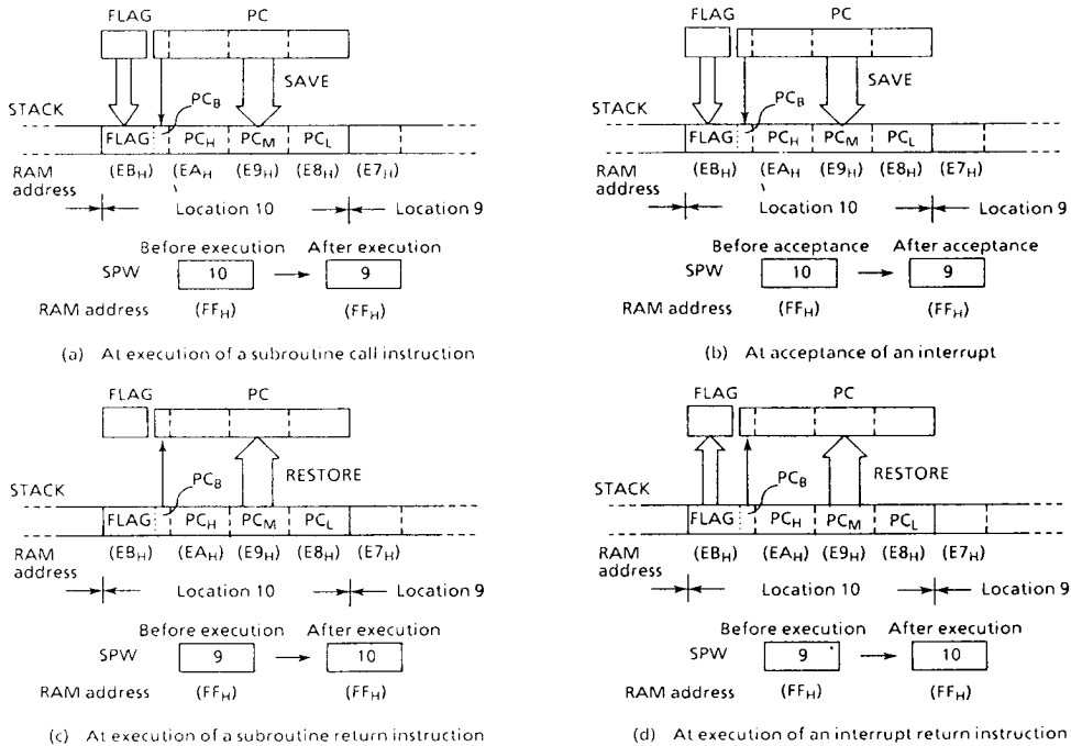
Figure 2-7. Accessing Stack (Save/Restore)
