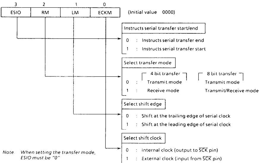
Figure 3-31. Serial Interface Control Command Register
