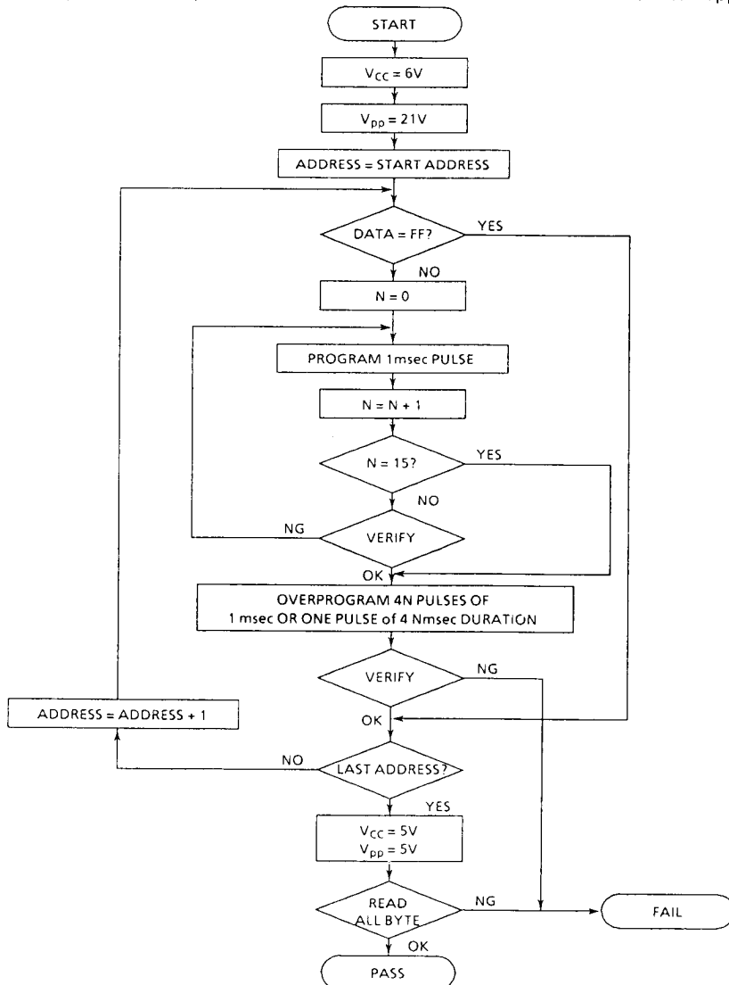
Figure1-4. FLOW CHART
