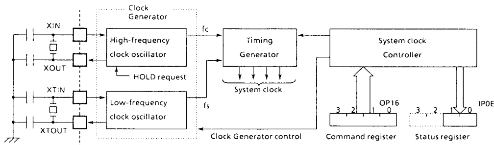
Figure 2-13. Clock Generator, Timing Generator and System Clock Controller
