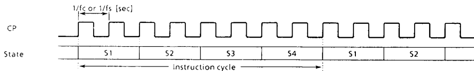
Figure 2-18. Instruction Cycle
