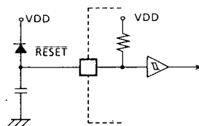
Figure 6-1. Simplified power-on-reset circuit
