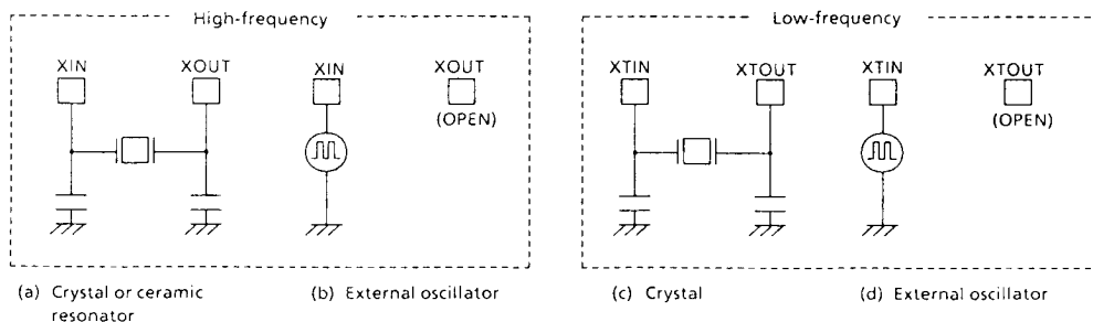
Figure 2-14. Examples of Resonator Connection
