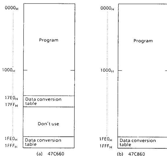
Figure 1-1. Program area
