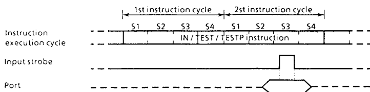
Figure 3-1. Input Timing
