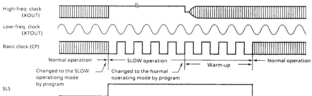
Figure 2-17. System Clock Switching Timing
