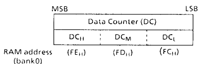
Figure 2-8. Data Counter
