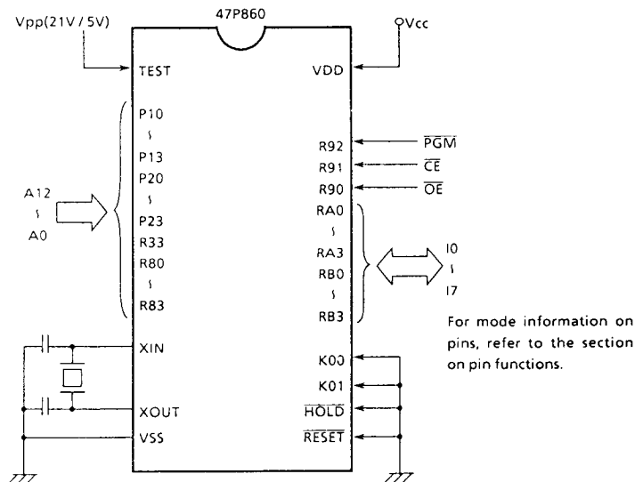
Figure 1-3. Setting for PROM mode
