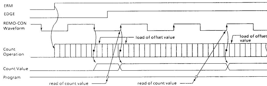
Figure 3-28. Timing chart
