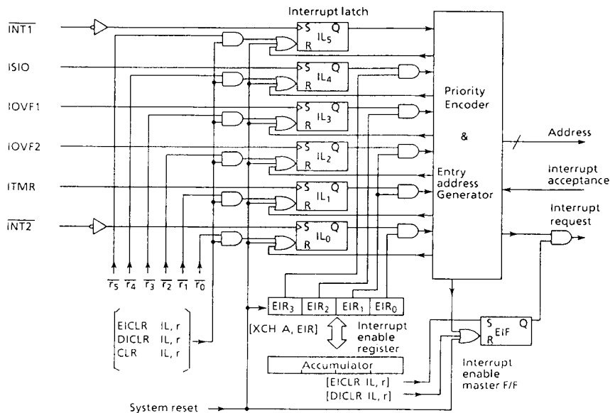
Figure 4-1. Interrupt Controller Block Diagram
