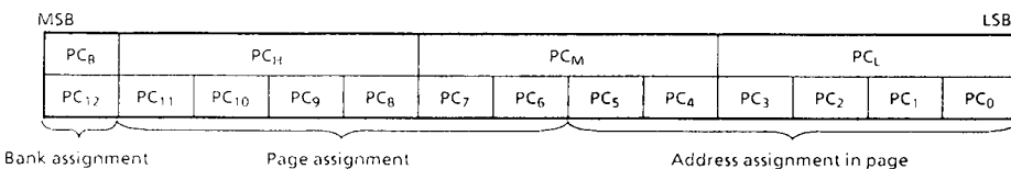
Figure 2-1. Configuration of Program Counter
