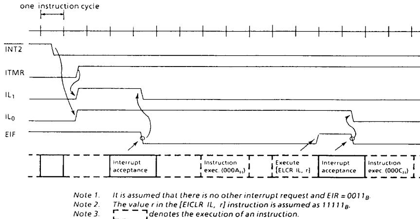
Figure 4-2. Interrupt Timing Chart (Example)
