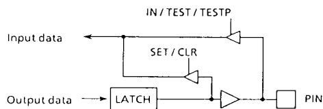
Figure 3-11. Ports RA, RB, RC
