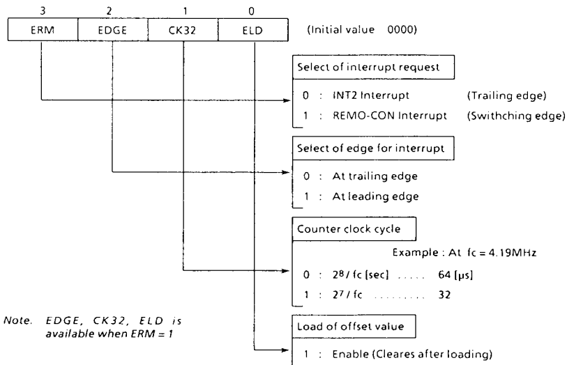
Figure 3-27. Command Register
