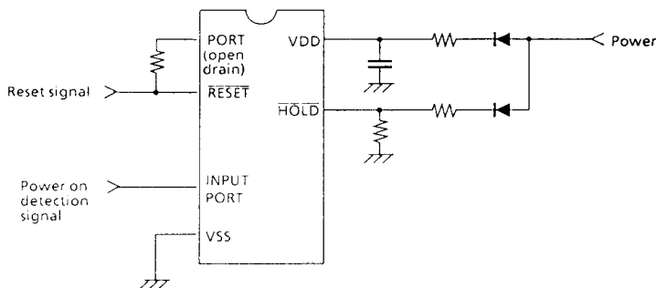
Figure 6-2. Warm-start Circuit Example
