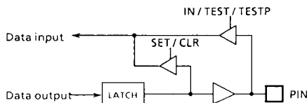
Figure 3-7. Port R6
