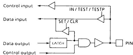
Figure 3-10. Port R9
