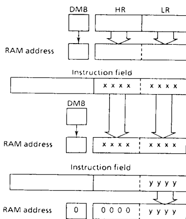
Figure 2-5. Addressing mode
