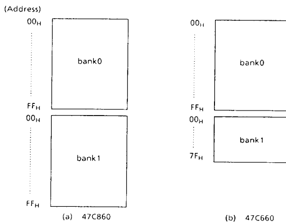
Figure 2-10. Data Memory (RAM)
