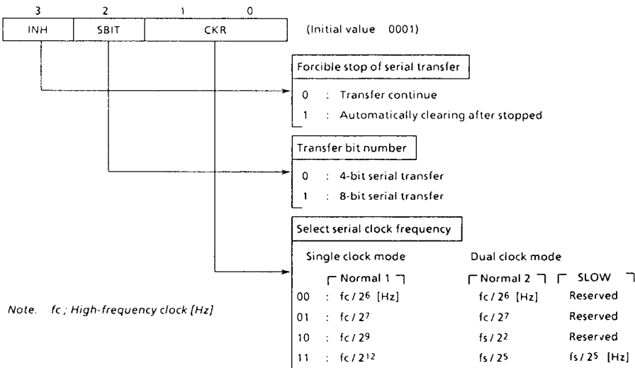
Serial interface control command register1 (port address OP1E)
