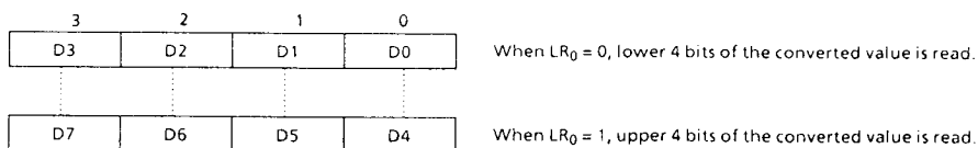
Figure 3-24. A/D converted value register
