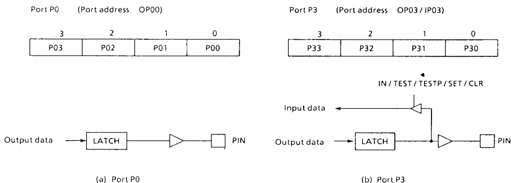
Figure 3-4. Ports P0, P3
