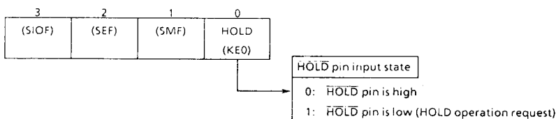
Figure 5-1. HOLD Operating Mode Command Register/Status Register
