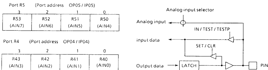
Figure 3-6. Ports R4, R5
