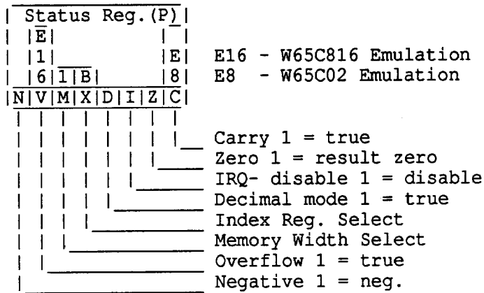
Figure 1-5 W65C832 Status Register Coding
