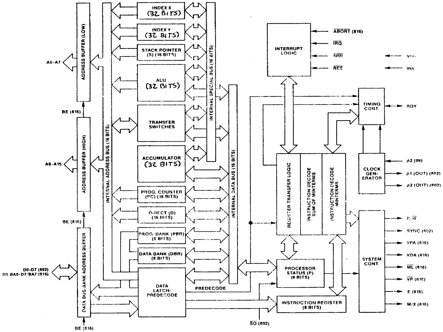
Figure 1-1 W65C832 Internal Architecture Simplified Block Diagram
