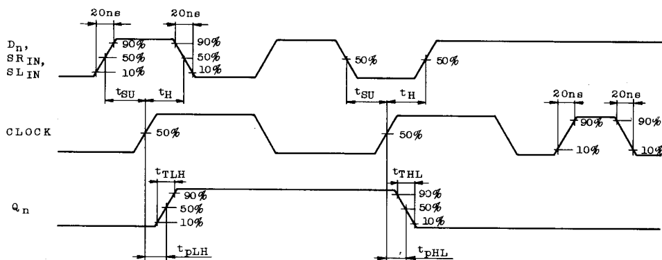
WAVEFORM 2
