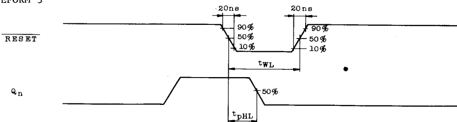
WAVEFORM 3
