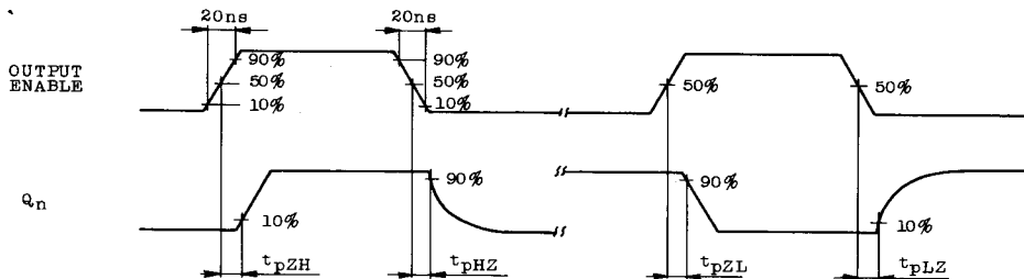
WAVEFORM 2
