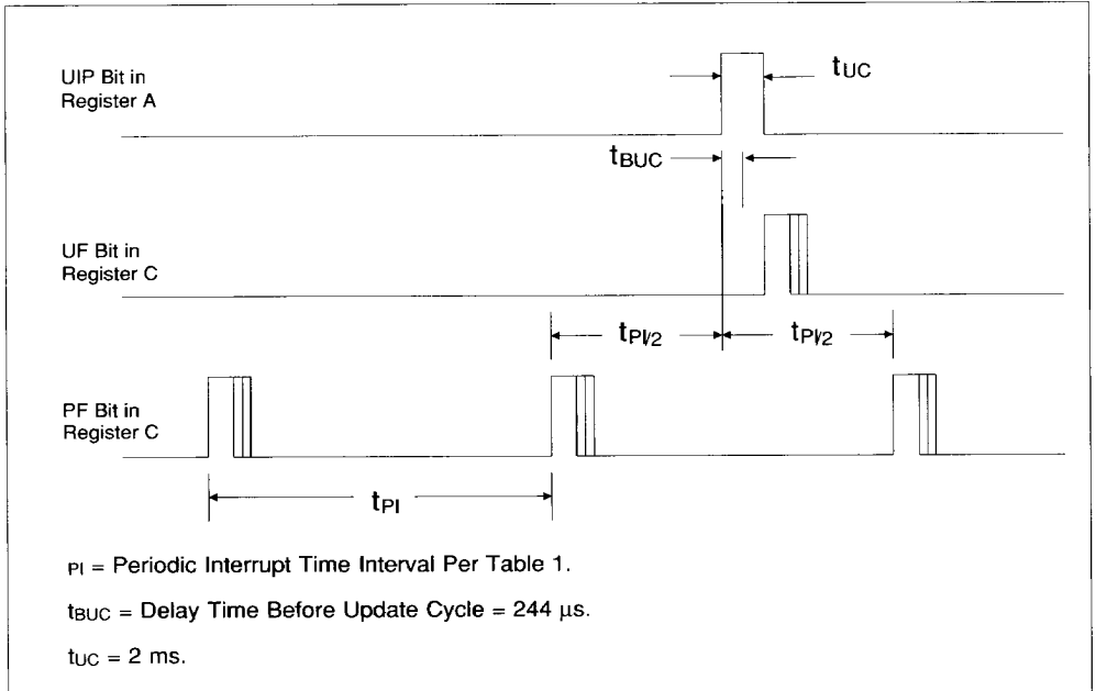
FIGURE 3 . UPDATE ENDED AND PERIODIC INTERRUPT RELATIONSHIP
