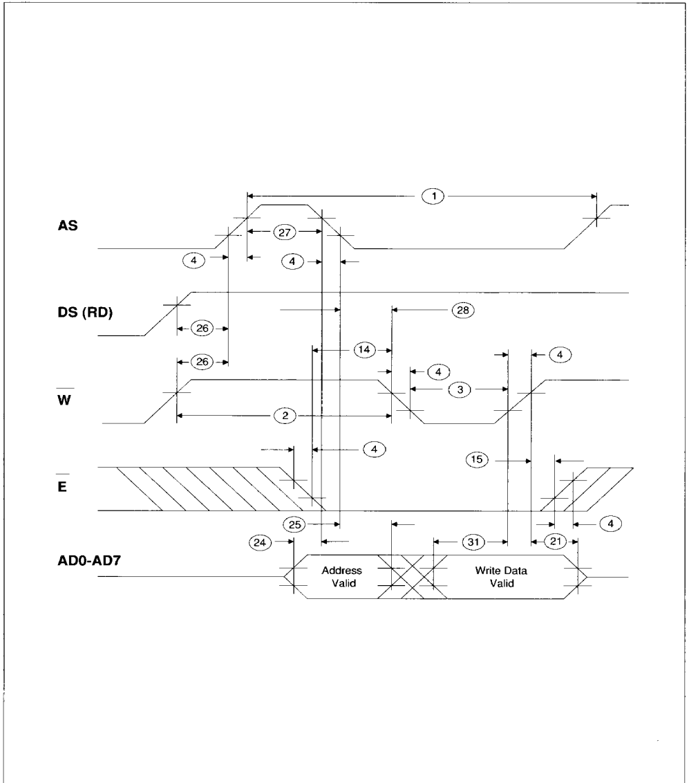
FIGURE 6 . BUS TIMING FOR INTEL INTERFACE WRITE CYCLE
