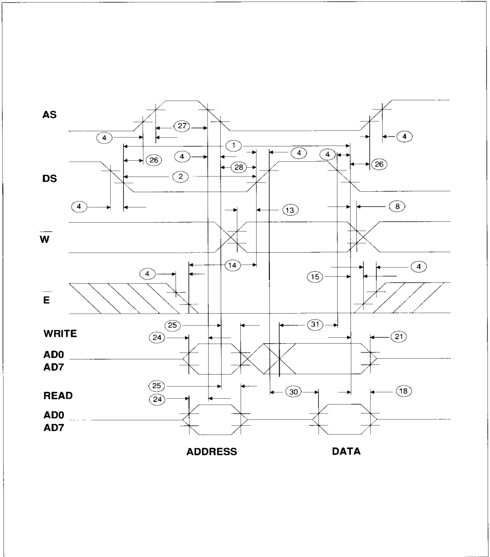
FIGURE 4 . BUS TIMING FOR MOTOROLA INTERFACE
