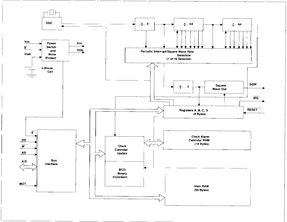
FIGURE 1 . BLOCK DIAGRAM
