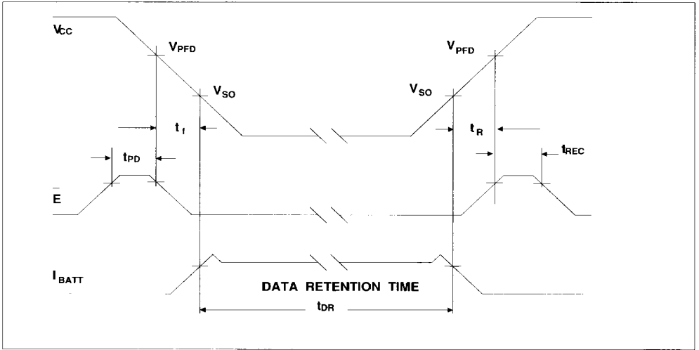
FIGURE 9 . POWER-UP / POWER-DOWN CONDITIONS
