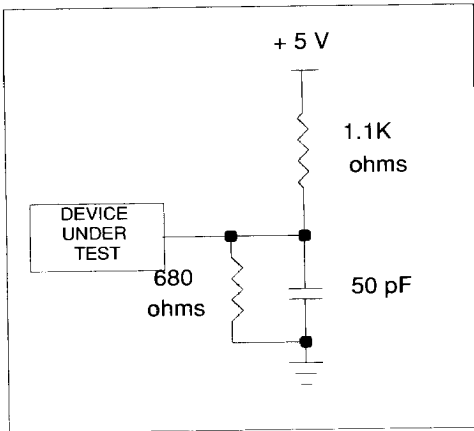
FIGURE 8 . OUTPUT LOAD
