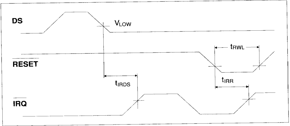
FIGURE 7 . IRQ RELEASE TIMING
