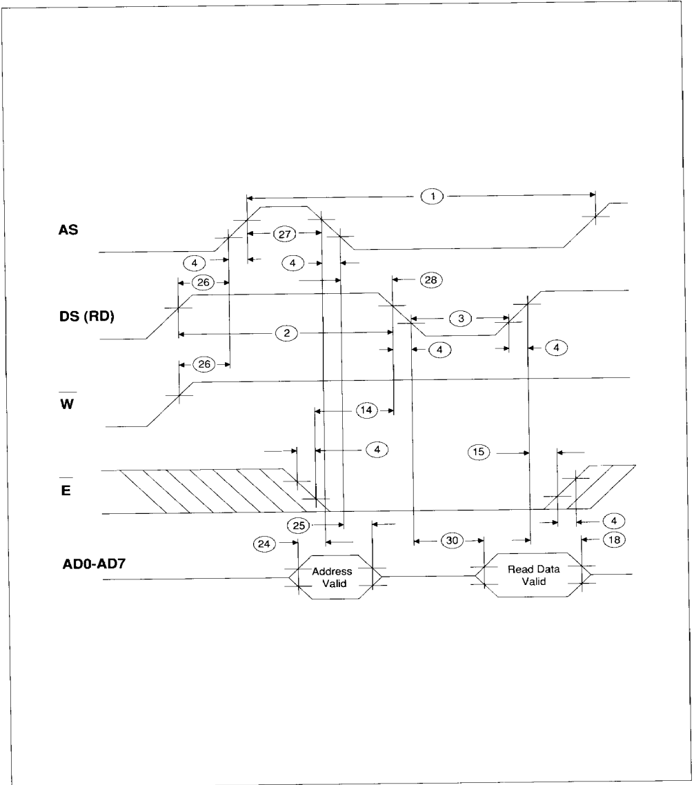
FIGURE 5. BUS TIMING FOR INTEL INTERFACE READ CYCLE
