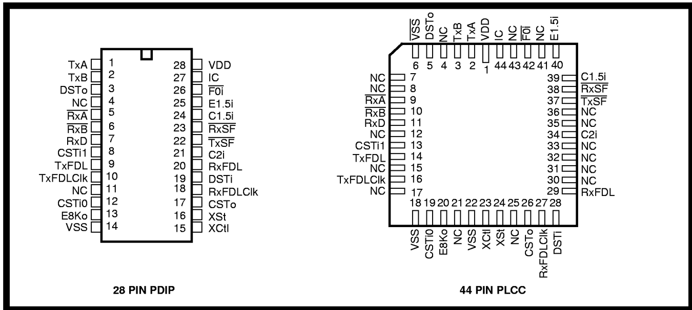
Figure 2 - Pin Connections
